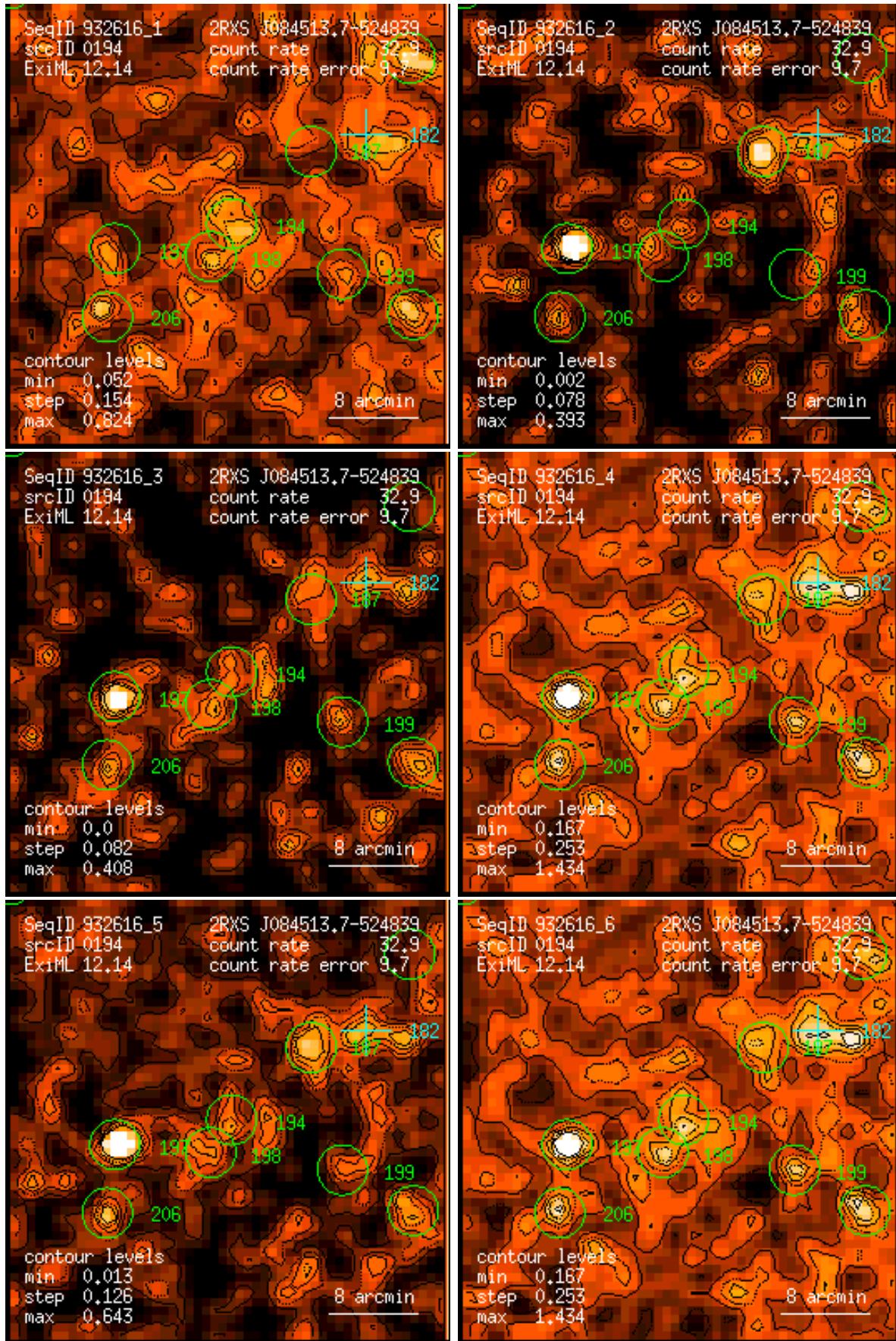
Figure 194: RASS 932616: detection 0194: band rate images, Gaussian filter: (1) PSPC channels 11 – 41, (2) 52 – 90, (3) 91 – 201, (4) 11 – 235, (5) 52 – 201, (6) 11 – 201. Broad band rates in counts/ks. Band rate contour levels in counts/ks/arcmin 2 .
