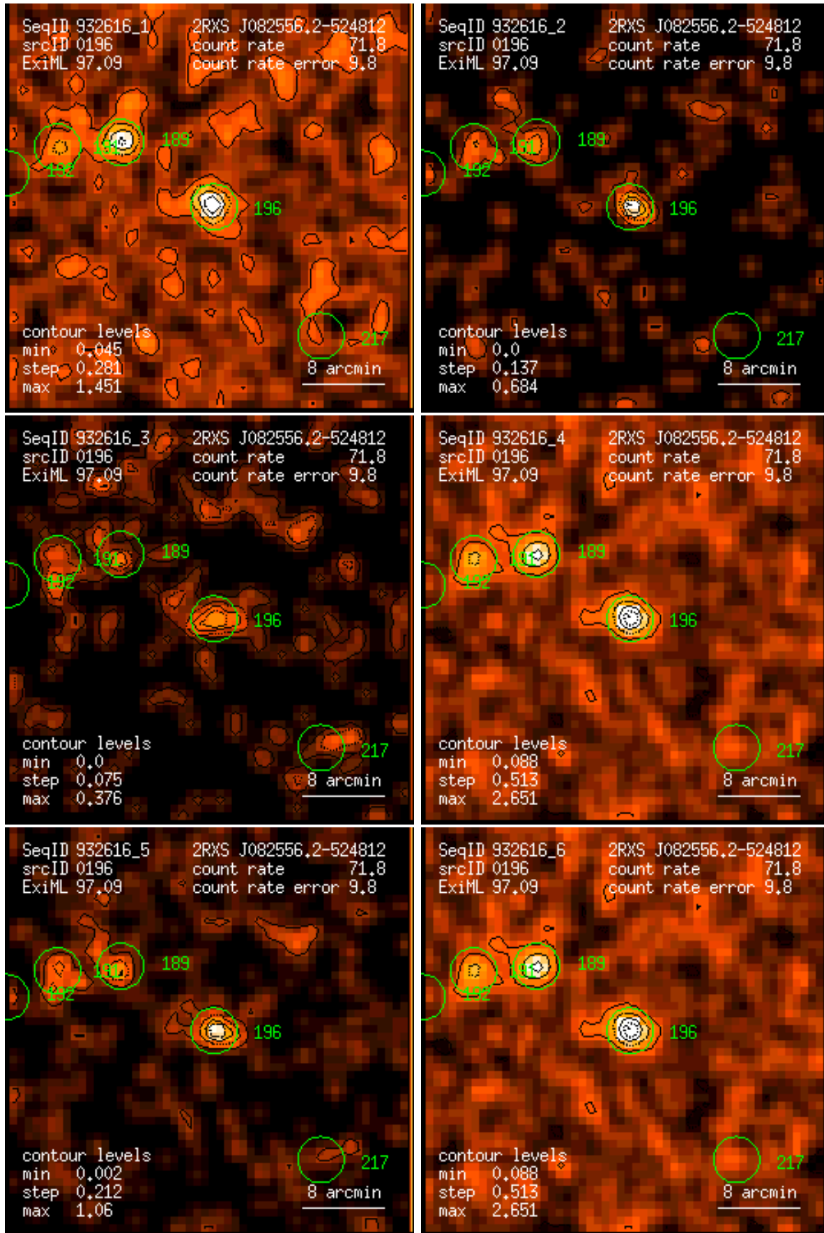
Figure 196: RASS 932616: detection 0196: band rate images, Gaussian filter: (1) PSPC channels 11 – 41, (2) 52 – 90, (3) 91 – 201, (4) 11 – 235, (5) 52 – 201, (6) 11 – 201. Broad band rates in counts/ks. Band rate contour levels in counts/ks/arcmin 2 .
