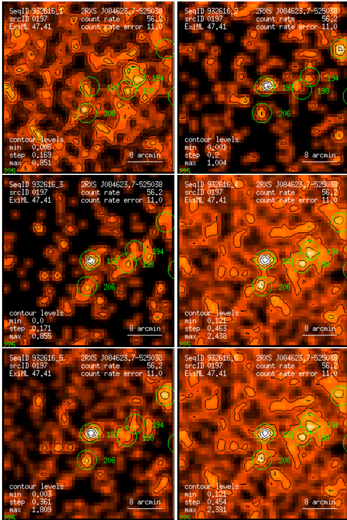
Figure 197: RASS 932616: detection 0197: band rate images, Gaussian filter: (1) PSPC channels 11 – 41, (2) 52 – 90, (3) 91 – 201, (4) 11 – 235, (5) 52 – 201, (6) 11 – 201. Broad band rates in counts/ks. Band rate contour levels in counts/ks/arcmin 2 .
