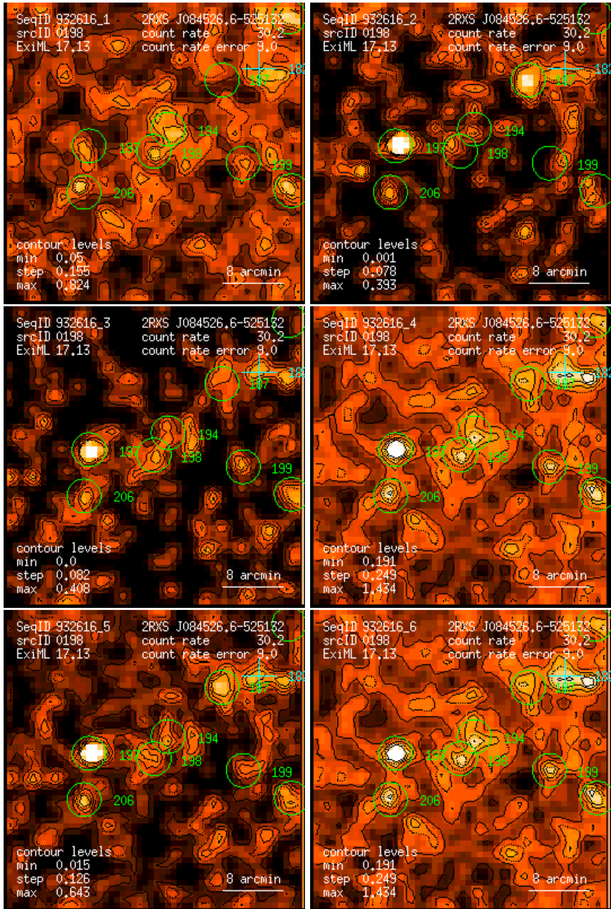
Figure 198: RASS 932616: detection 0198: band rate images, Gaussian filter: (1) PSPC channels 11 – 41, (2) 52 – 90, (3) 91 – 201, (4) 11 – 235, (5) 52 – 201, (6) 11 – 201. Broad band rates in counts/ks. Band rate contour levels in counts/ks/arcmin 2 .
