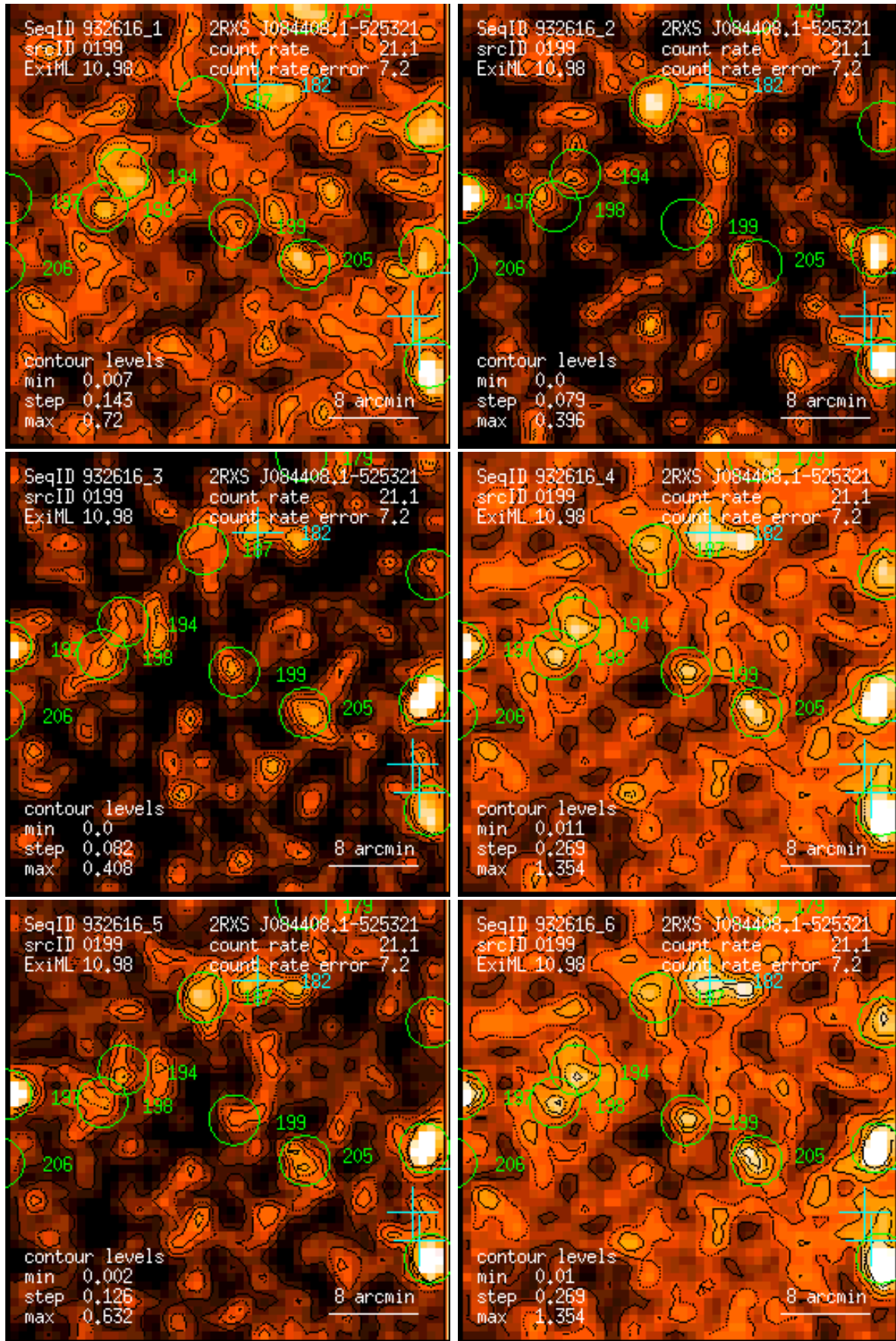
Figure 199: RASS 932616: detection 0199: band rate images, Gaussian filter: (1) PSPC channels 11 – 41, (2) 52 – 90, (3) 91 – 201, (4) 11 – 235, (5) 52 – 201, (6) 11 – 201. Broad band rates in counts/ks. Band rate contour levels in counts/ks/arcmin 2 .
