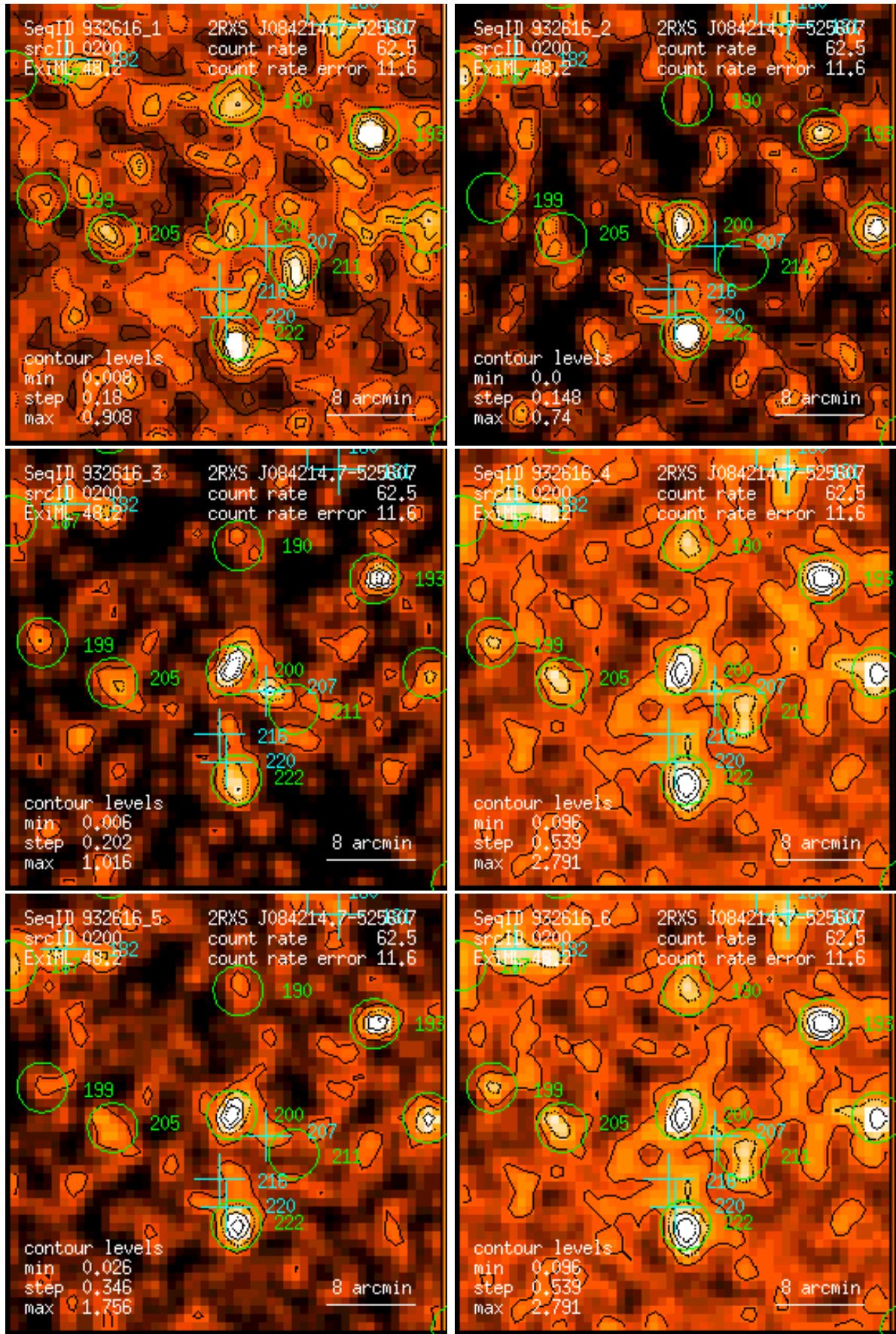
Figure 200: RASS 932616: detection 0200: band rate images, Gaussian filter: (1) PSPC channels 11 – 41, (2) 52 – 90, (3) 91 – 201, (4) 11 – 235, (5) 52 – 201, (6) 11 – 201. Broad band rates in counts/ks. Band rate contour levels in counts/ks/arcmin 2 .
