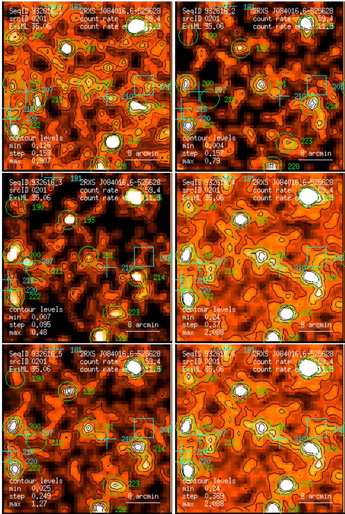
Figure 201: RASS 932616: detection 0201: band rate images, Gaussian filter: (1) PSPC channels 11 – 41, (2) 52 – 90, (3) 91 – 201, (4) 11 – 235, (5) 52 – 201, (6) 11 – 201. Broad band rates in counts/ks. Band rate contour levels in counts/ks/arcmin 2 .
