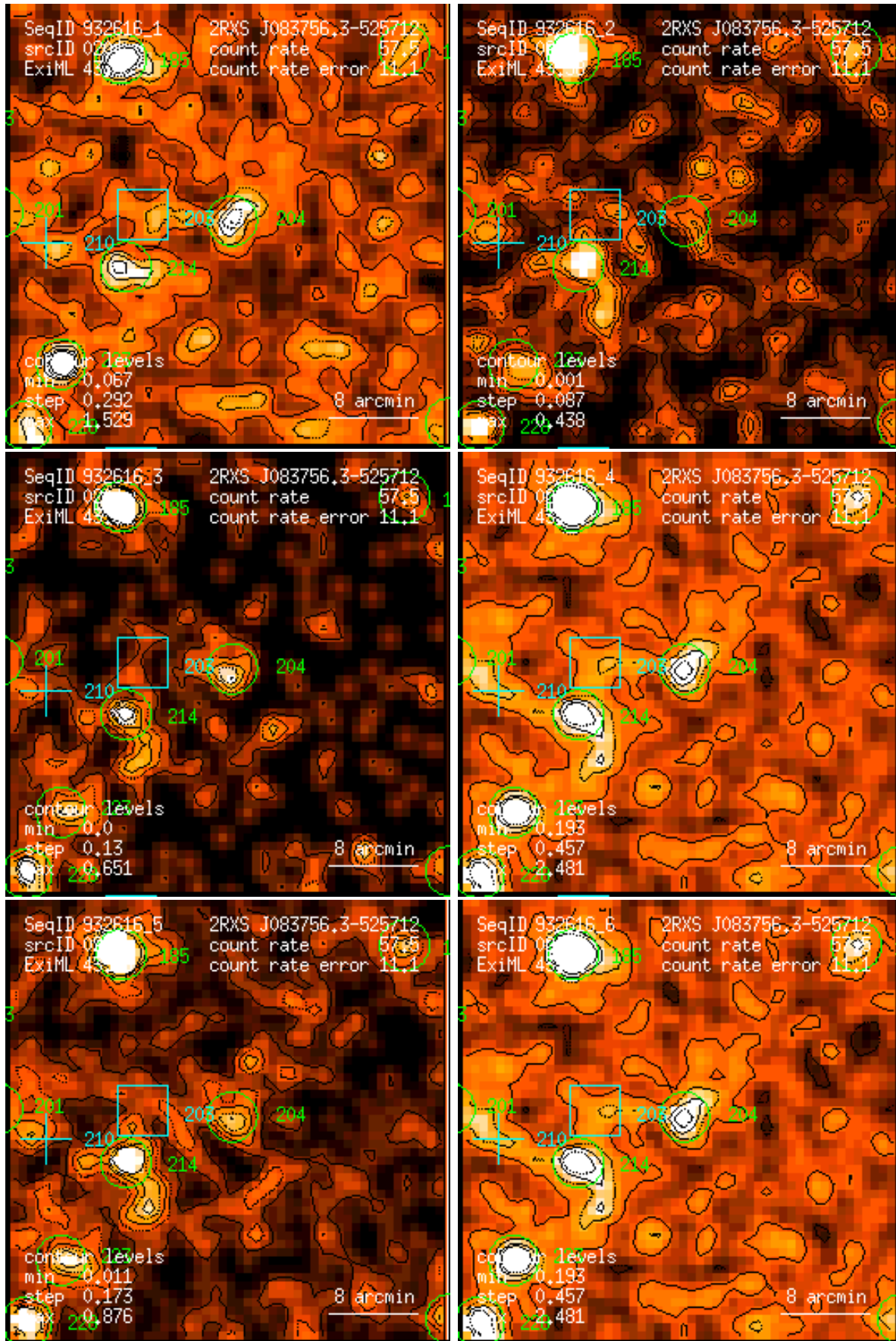
Figure 204: RASS 932616: detection 0204: band rate images, Gaussian filter: (1) PSPPC channels 11 – 41, (2) 52 – 90, (3) 91 – 201, (4) 11 – 235, (5) 52 – 201, (6) 11 – 201. Broad band rates in counts/ks. Band rate contour levels in counts/ks/arcmin 2 .
