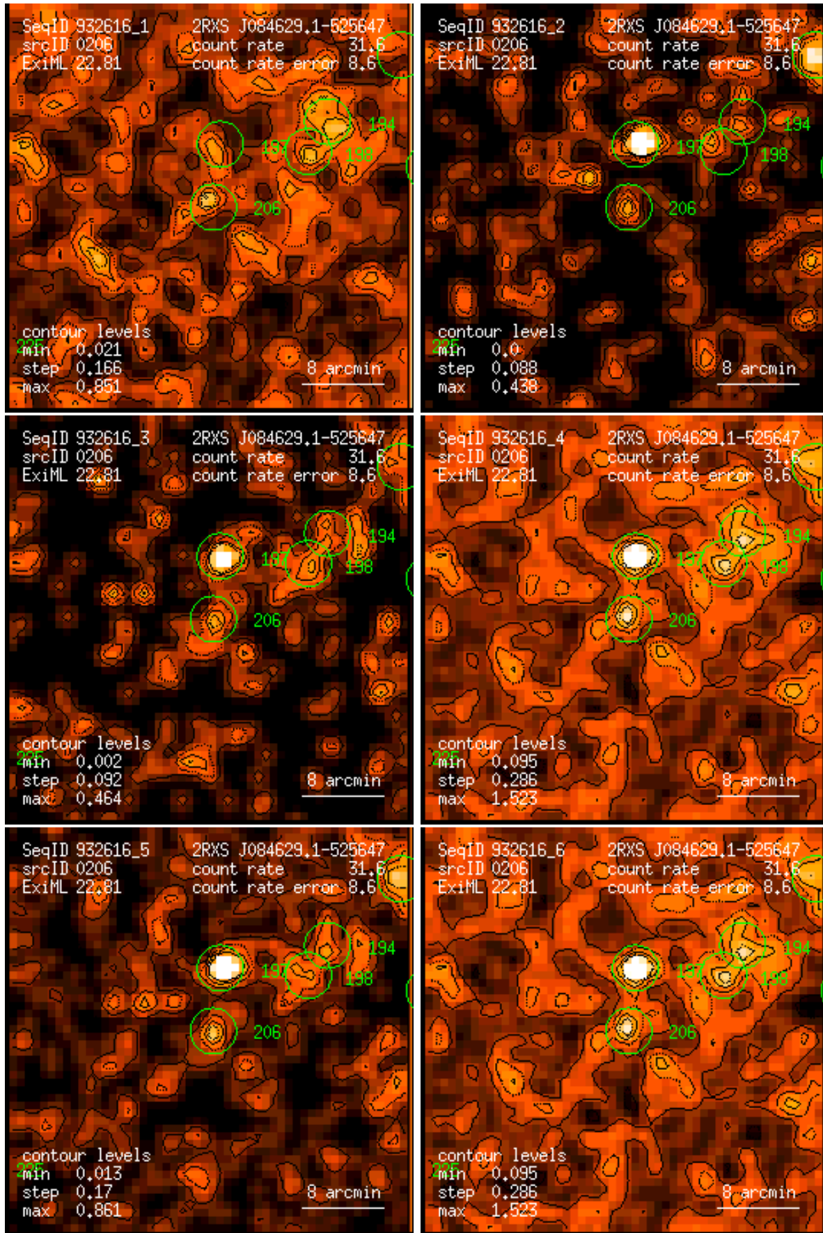
Figure 206: RASS 932616: detection 0206: band rate images, Gaussian filter: (1) PSPC channels 11 – 41, (2) 52 – 90, (3) 91 – 201, (4) 11 – 235, (5) 52 – 201, (6) 11 – 201. Broad band rates in counts/ks. Band rate contour levels in counts/ks/arcmin 2 .
