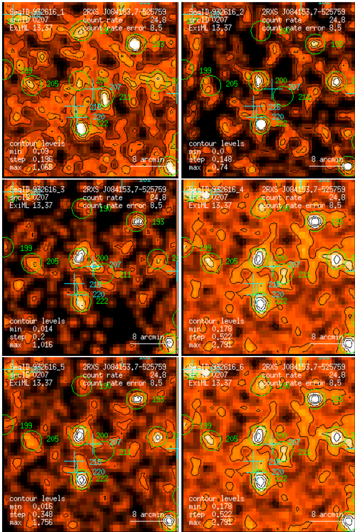
Figure 207: RASS 932616: detection 0207: band rate images, Gaussian filter: (1) PSPC channels 11 – 41, (2) 52 – 90, (3) 91 – 201, (4) 11 – 235, (5) 52 – 201, (6) 11 – 201. Broad band rates in counts/ks. Band rate contour levels in counts/ks/arcmin 2 .
