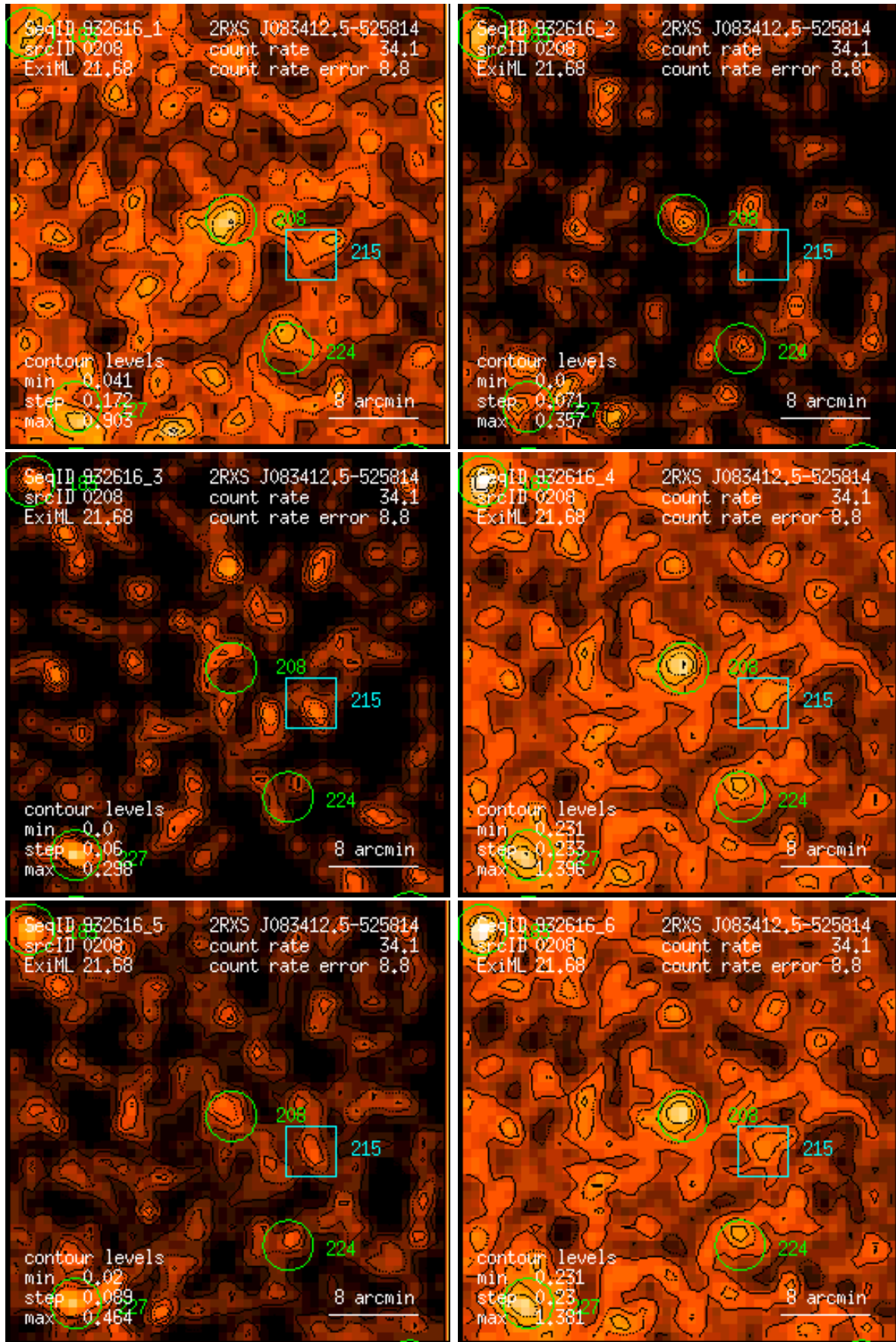
Figure 208: RASS 932616: detection 0208: band rate images, Gaussian filter: (1) PSPC channels 11 – 41, (2) 52 – 90, (3) 91 – 201, (4) 11 – 235, (5) 52 – 201, (6) 11 – 201. Broad band rates in counts/ks. Band rate contour levels in counts/ks/arcmin 2 .
