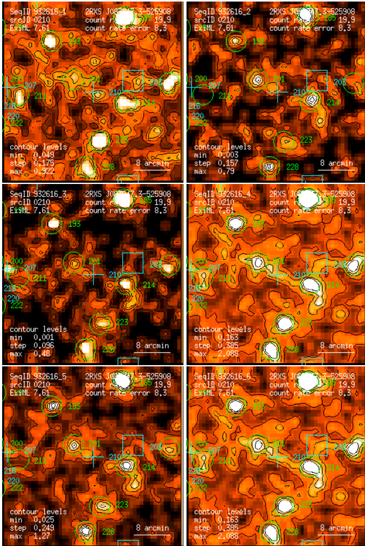
Figure 210: RASS 932616: detection 0210: band rate images, Gaussian filter: (1) PSPC channels 11 – 41, (2) 52 – 90, (3) 91 – 201, (4) 11 – 235, (5) 52 – 201, (6) 11 – 201. Broad band rates in counts/ks. Band rate contour levels in counts/ks/arcmin 2 .
