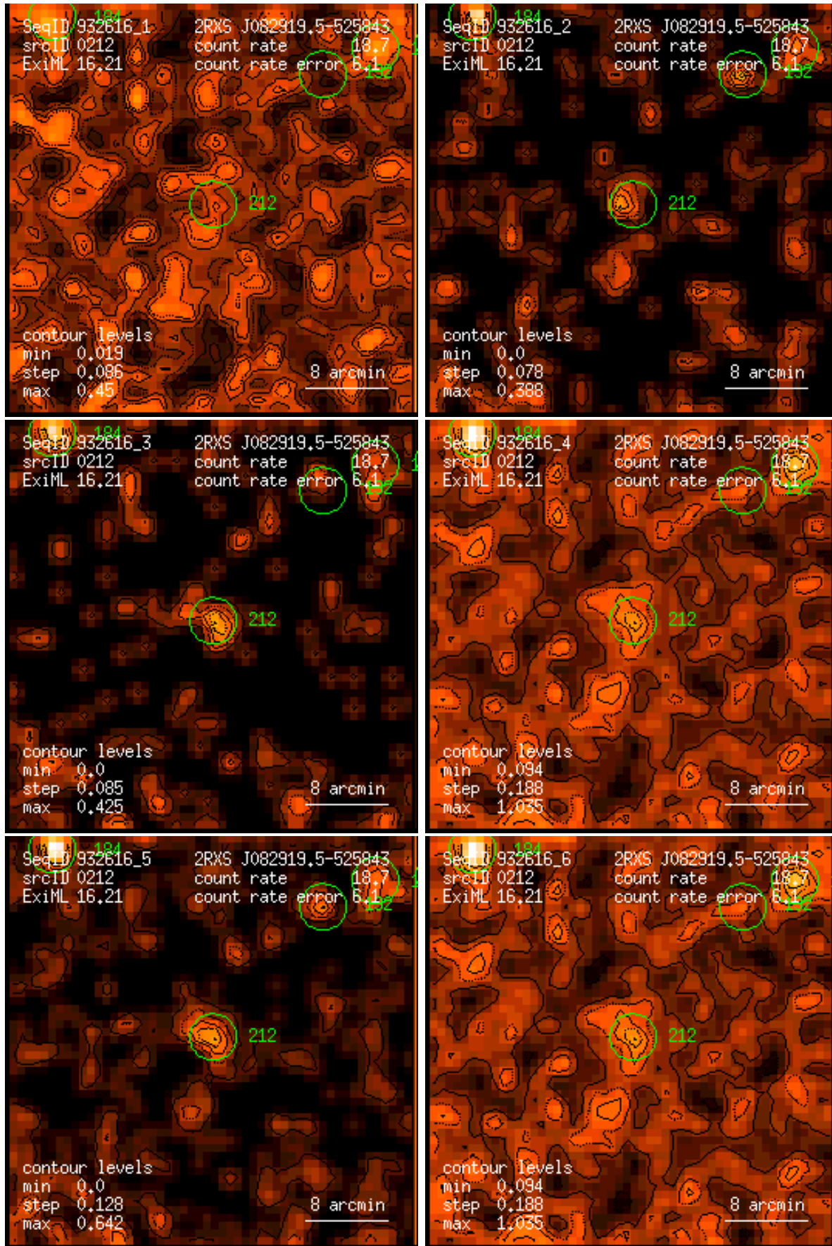
Figure 212: RASS 932616: detection 0212: band rate images, Gaussian filter: (1) PSPC channels 11 – 41, (2) 52 – 90, (3) 91 – 201, (4) 11 – 235, (5) 52 – 201, (6) 11 – 201. Broad band rates in counts/ks. Band rate contour levels in counts/ks/arcmin 2 .
