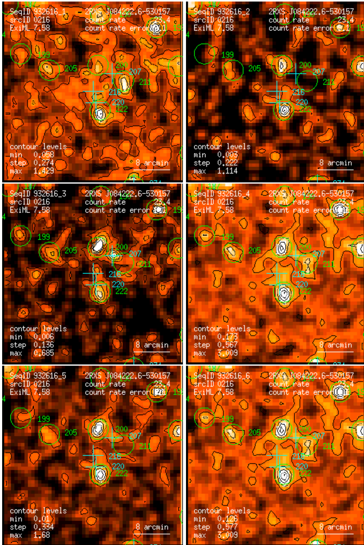
Figure 216: RASS 932616: detection 0216: band rate images, Gaussian filter: (1) PSPC channels 11 – 41, (2) 52 – 90, (3) 91 – 201, (4) 11 – 235, (5) 52 – 201, (6) 11 – 201. Broad band rates in counts/ks. Band rate contour levels in counts/ks/arcmin 2 .
