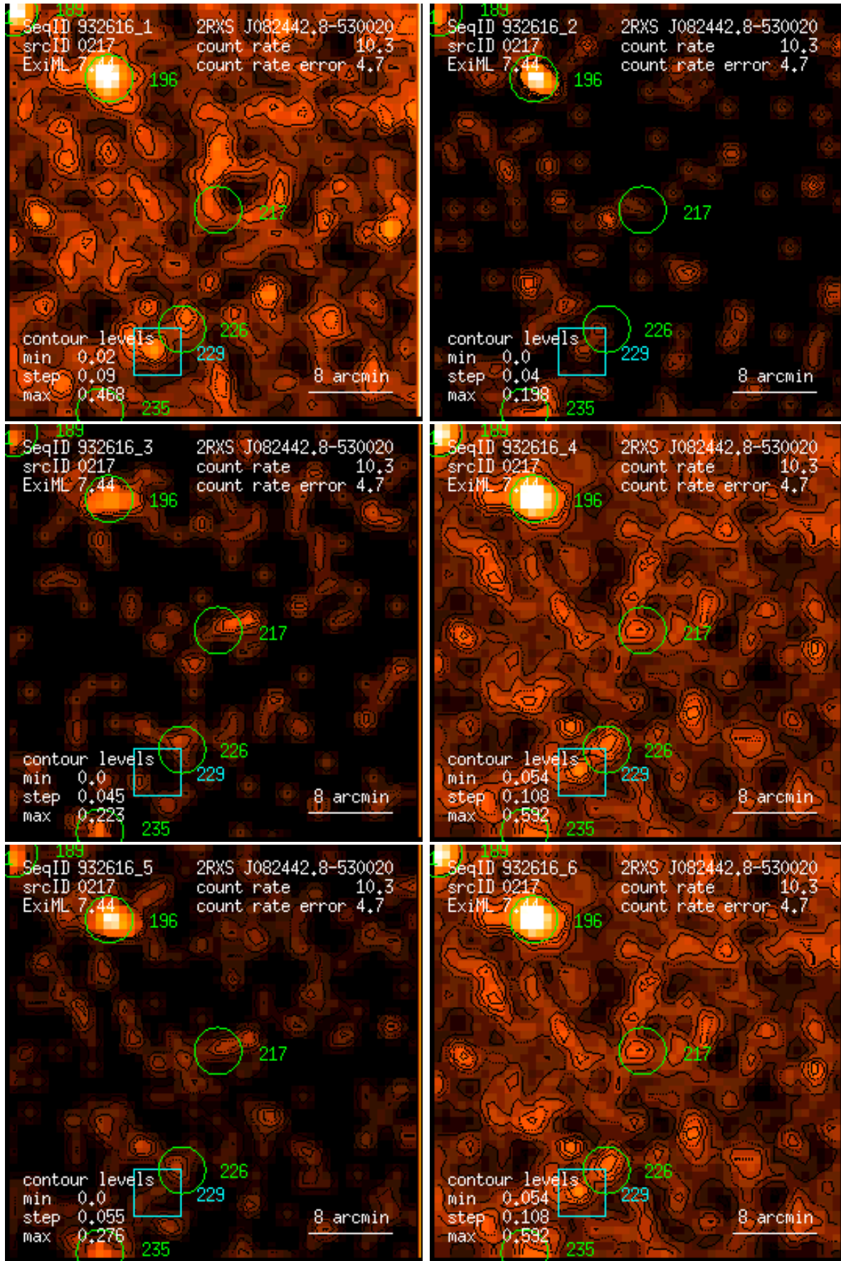
Figure 217: RASS 932616: detection 0217: band rate images, Gaussian filter: (1) PSPC channels 11 – 41, (2) 52 – 90, (3) 91 – 201, (4) 11 – 235, (5) 52 – 201, (6) 11 – 201. Broad band rates in counts/ks. Band rate contour levels in counts/ks/arcmin 2 .
