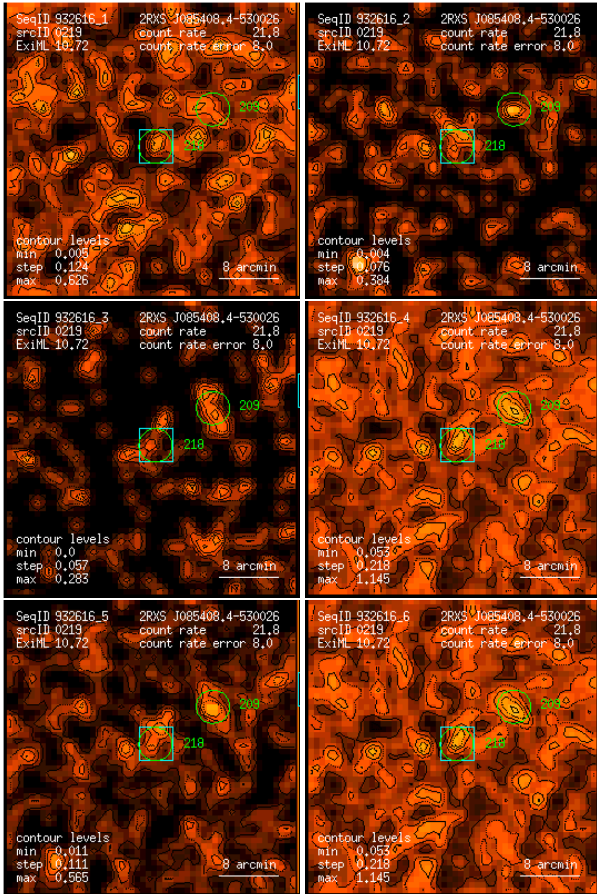
Figure 219: RASS 932616: detection 0219: band rate images, Gaussian filter: (1) PSPC channels 11 – 41, (2) 52 – 90, (3) 91 – 201, (4) 11 – 235, (5) 52 – 201, (6) 11 – 201. Broad band rates in counts/ks. Band rate contour levels in counts/ks/arcmin 2 .
