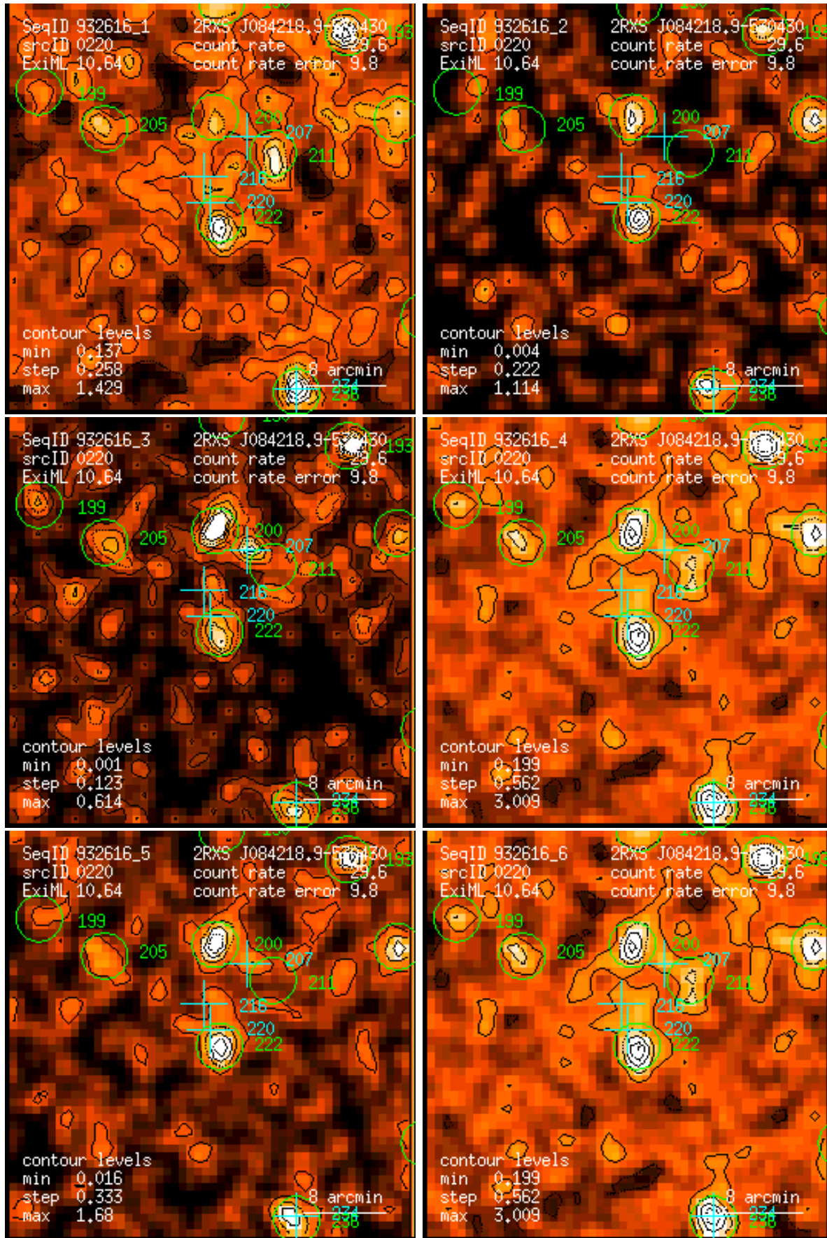
Figure 220: RASS 932616: detection 0220: band rate images, Gaussian filter: (1) PSPC channels 11 – 41, (2) 52 – 90, (3) 91 – 201, (4) 11 – 235, (5) 52 – 201, (6) 11 – 201. Broad band rates in counts/ks. Band rate contour levels in counts/ks/arcmin 2 .
