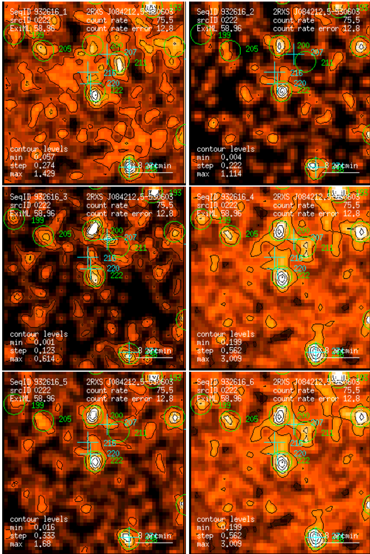
Figure 222: RASS 932616: detection 0222: band rate images, Gaussian filter: (1) PSPC channels 11 – 41, (2) 52 – 90, (3) 91 – 201, (4) 11 – 235, (5) 52 – 201, (6) 11 – 201. Broad band rates in counts/ks. Band rate contour levels in counts/ks/arcmin 2 .
