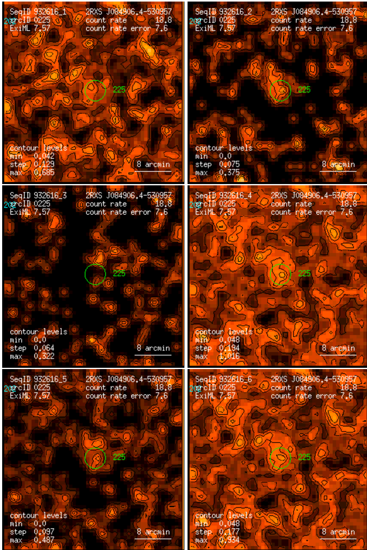
Figure 225: RASS 932616: detection 0225: band rate images, Gaussian filter: (1) PSPC channels 11 – 41, (2) 52 – 90, (3) 91 – 201, (4) 11 – 235, (5) 52 – 201, (6) 11 – 201. Broad band rates in counts/ks. Band rate contour levels in counts/ks/arcmin 2 .
