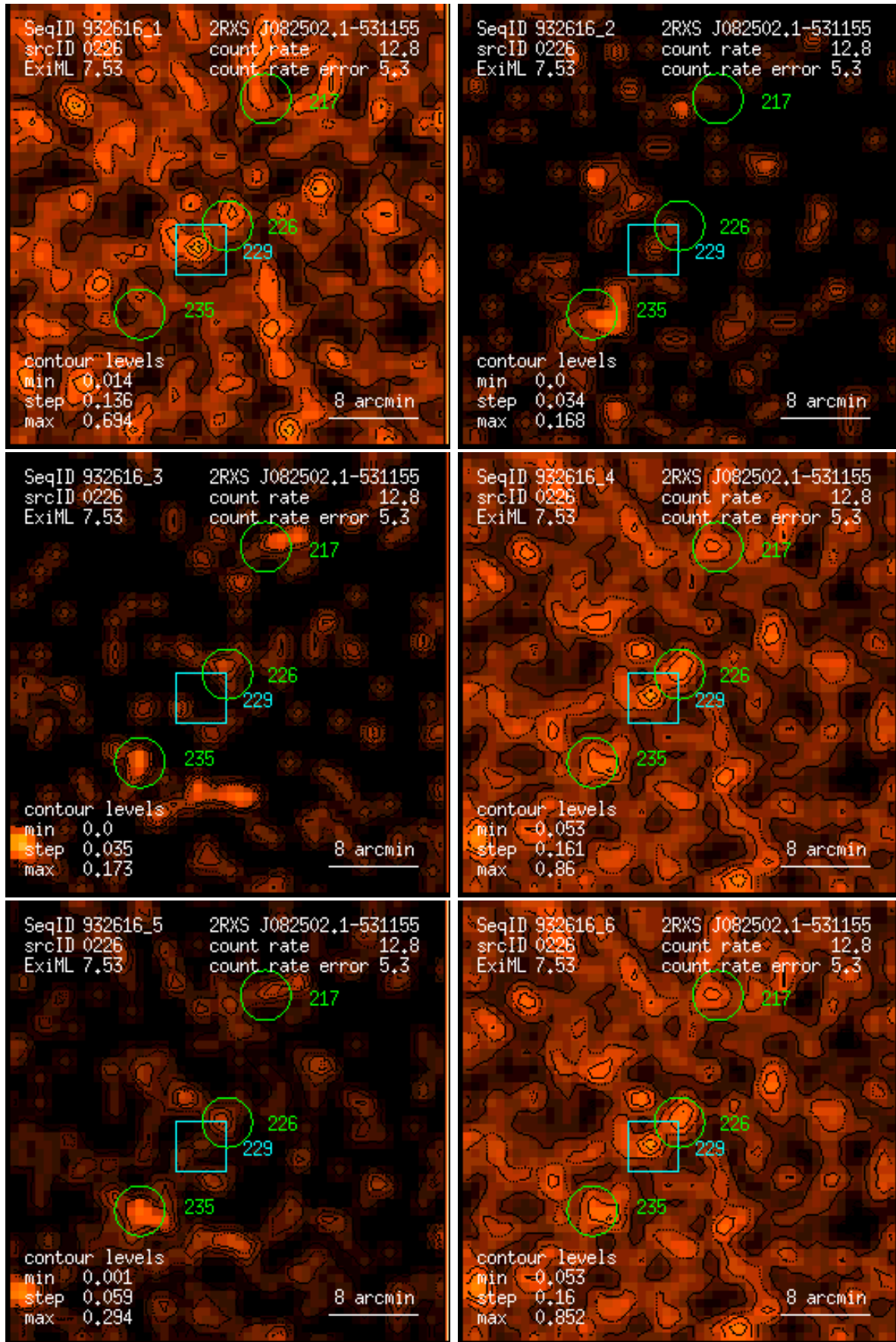
Figure 226: RASS 932616: detection 0226: band rate images, Gaussian filter: (1) PSPC channels 11 – 41, (2) 52 – 90, (3) 91 – 201, (4) 11 – 235, (5) 52 – 201, (6) 11 – 201. Broad band rates in counts/ks. Band rate contour levels in counts/ks/arcmin 2 .
