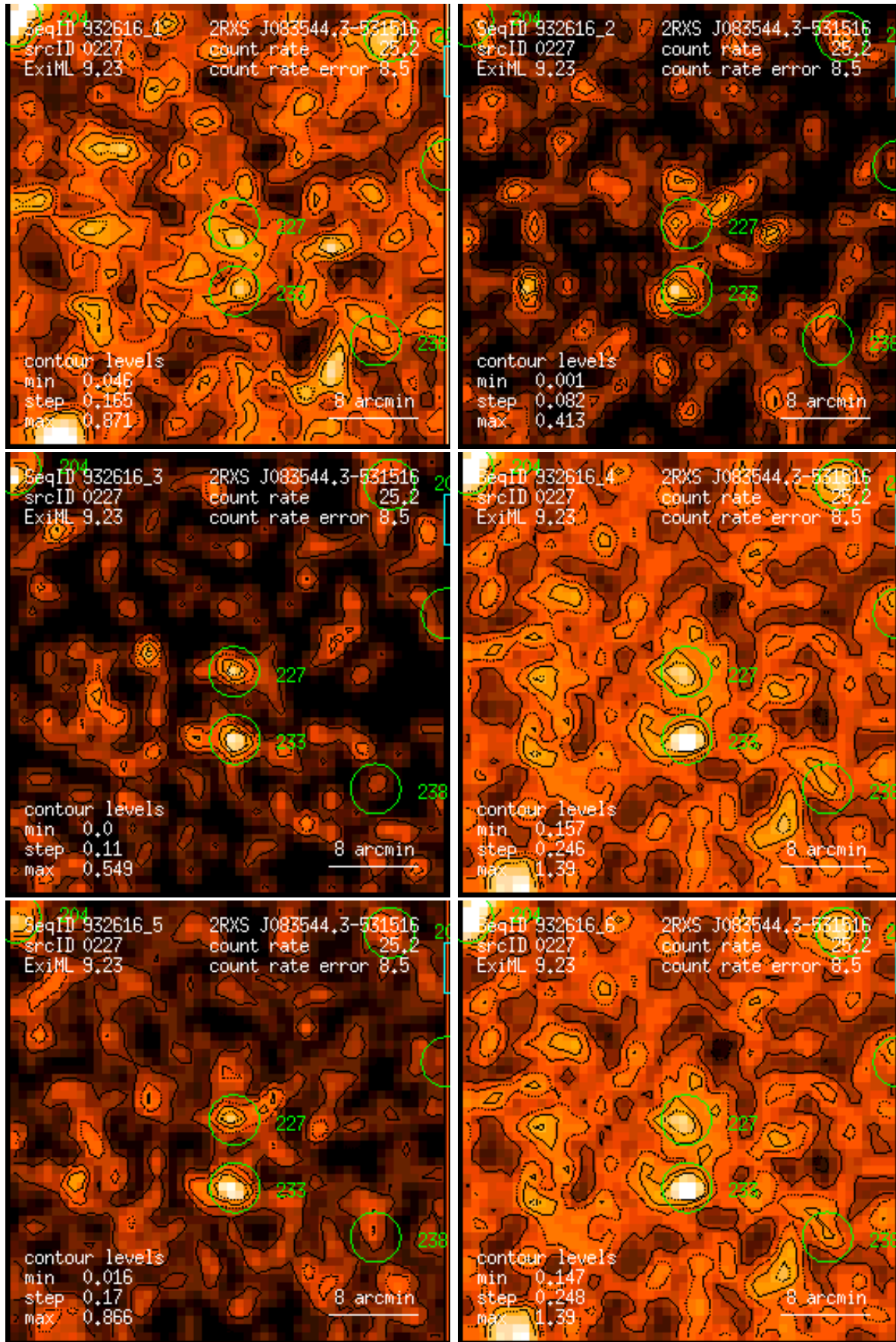
Figure 227: RASS 932616: detection 0227: band rate images, Gaussian filter: (1) PSPC channels 11 – 41, (2) 52 – 90, (3) 91 – 201, (4) 11 – 235, (5) 52 – 201, (6) 11 – 201. Broad band rates in counts/ks. Band rate contour levels in counts/ks/arcmin 2 .
