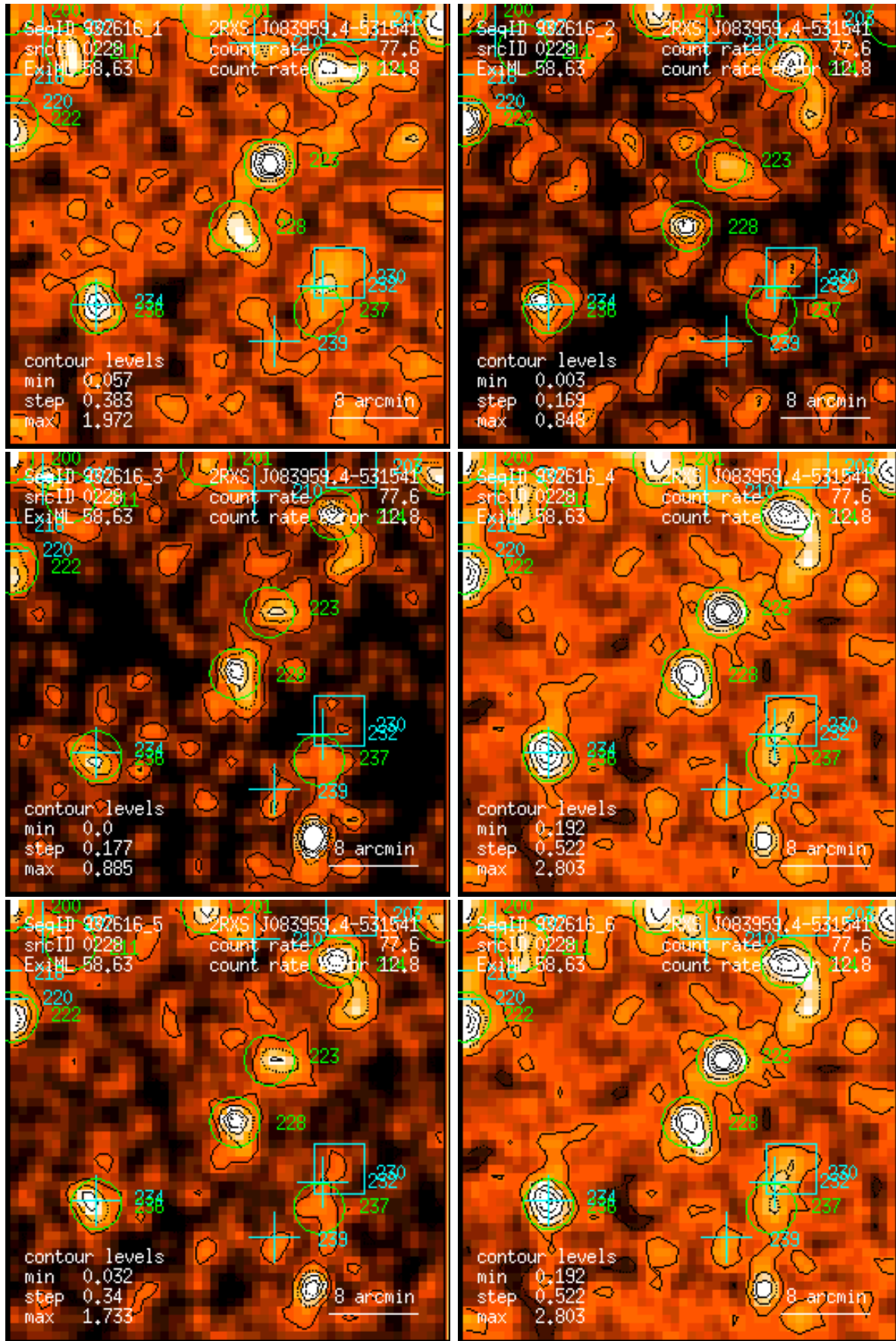
Figure 228: RASS 932616: detection 0228: band rate images, Gaussian filter: (1) PSPC channels 11 – 41, (2) 52 – 90, (3) 91 – 201, (4) 11 – 235, (5) 52 – 201, (6) 11 – 201. Broad band rates in counts/ks. Band rate contour levels in counts/ks/arcmin 2 .
