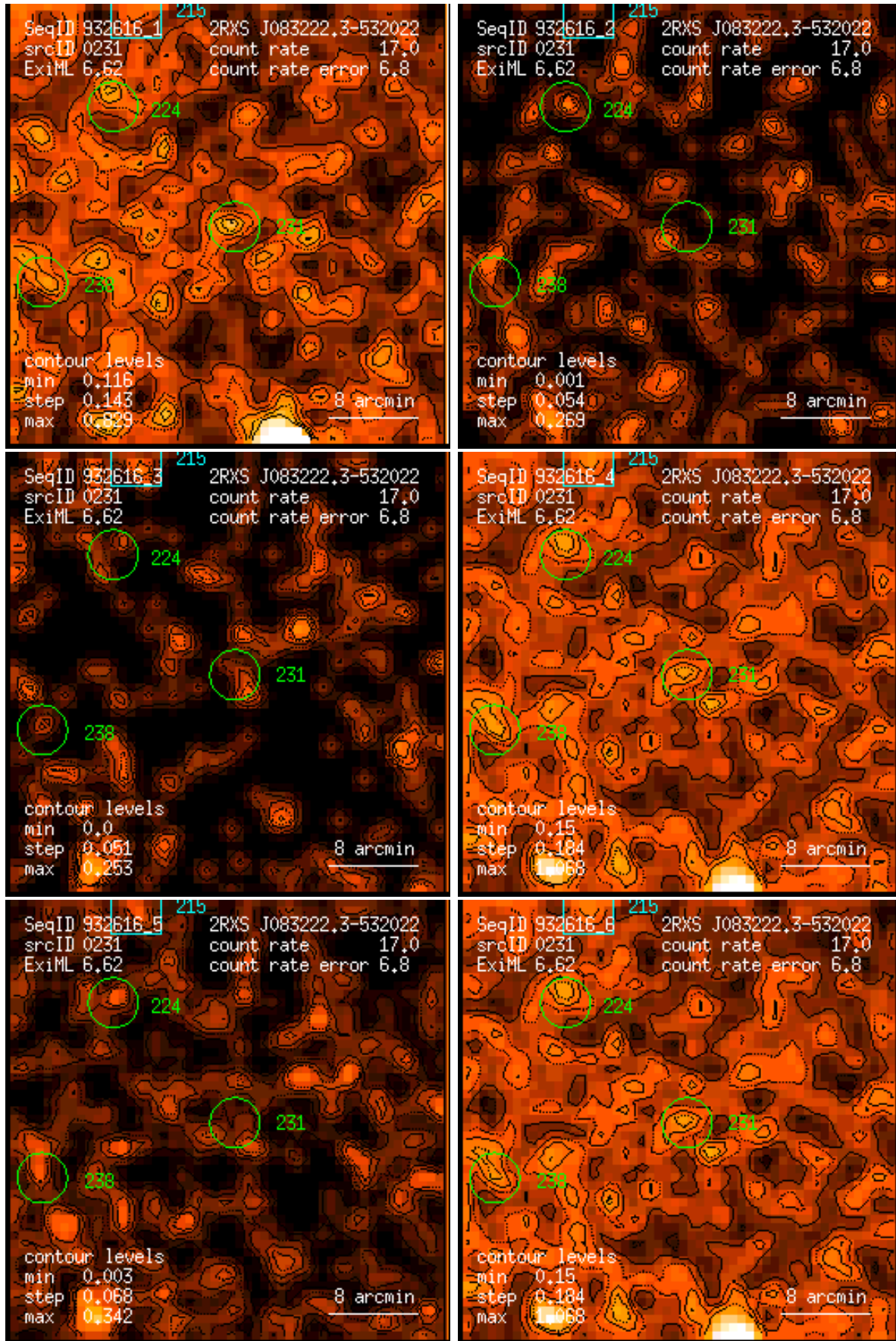
Figure 231: RASS 932616: detection 0231: band rate images, Gaussian filter: (1) PSPC channels 11 – 41, (2) 52 – 90, (3) 91 – 201, (4) 11 – 235, (5) 52 – 201, (6) 11 – 201. Broad band rates in counts/ks. Band rate contour levels in counts/ks/arcmin 2 .
