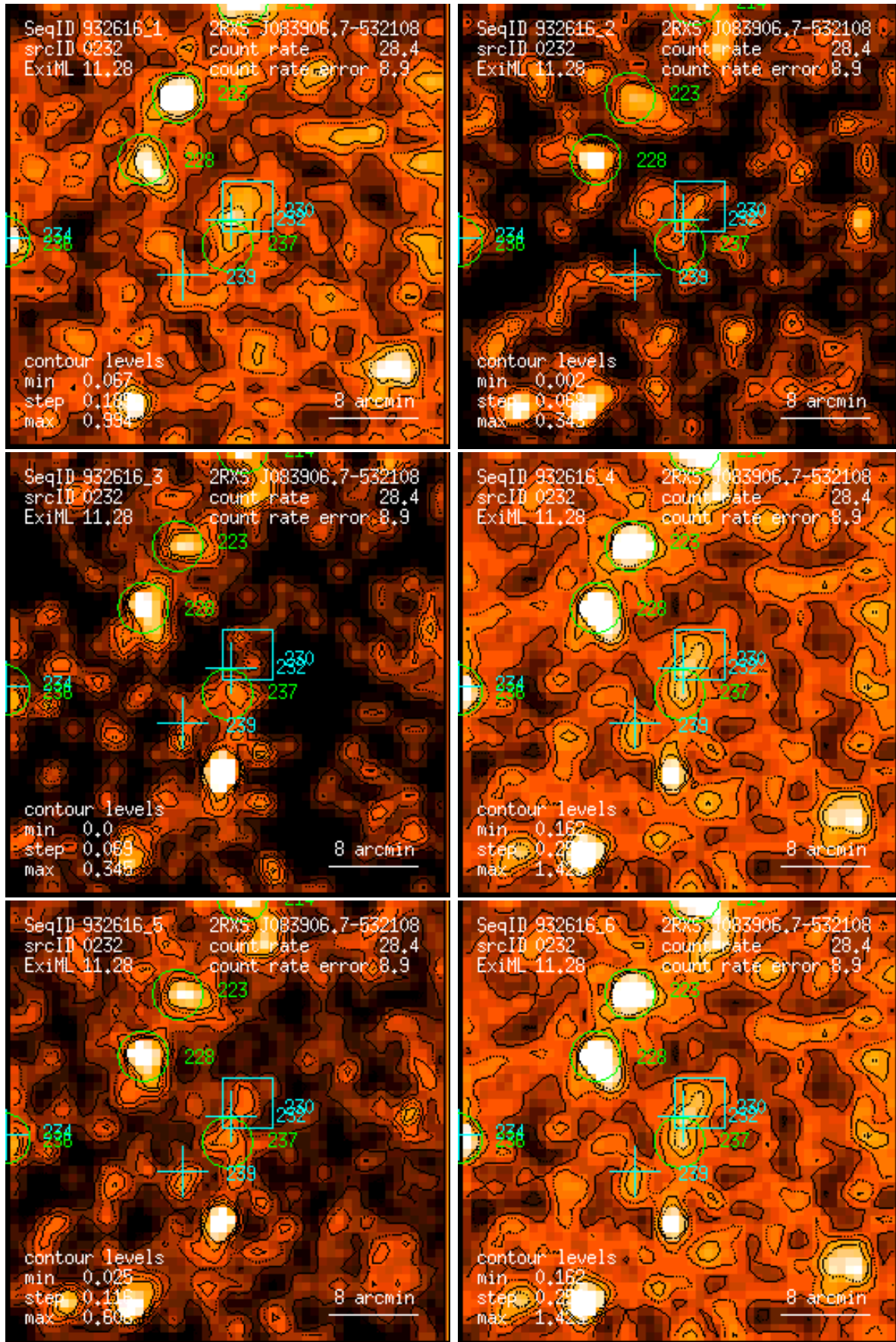
Figure 232: RASS 932616: detection 0232: band rate images, Gaussian filter: (1) PSPC channels 11 – 41, (2) 52 – 90, (3) 91 – 201, (4) 11 – 235, (5) 52 – 201, (6) 11 – 201. Broad band rates in counts/ks. Band rate contour levels in counts/ks/arcmin 2 .
