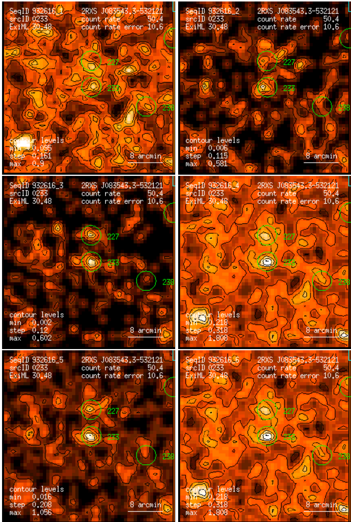
Figure 233: RASS 932616: detection 0233: band rate images, Gaussian filter: (1) PSPC channels 11 – 41, (2) 52 – 90, (3) 91 – 201, (4) 11 – 235, (5) 52 – 201, (6) 11 – 201. Broad band rates in counts/ks. Band rate contour levels in counts/ks/arcmin 2 .
