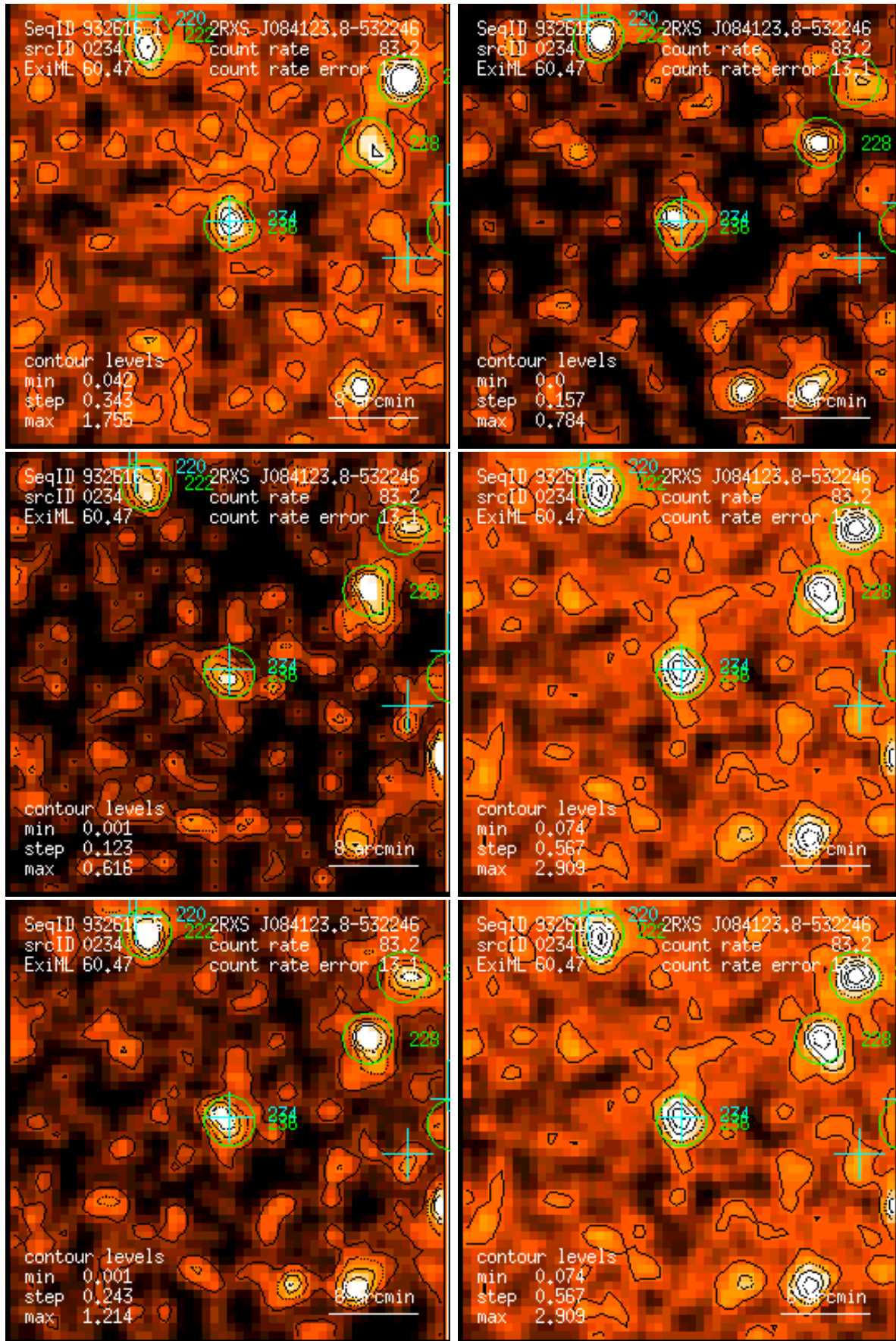
Figure 234: RASS 932616: detection 0234: band rate images, Gaussian filter: (1) PSPC channels 11 – 41, (2) 52 – 90, (3) 91 – 201, (4) 11 – 235, (5) 52 – 201, (6) 11 – 201. Broad band rates in counts/ks. Band rate contour levels in counts/ks/arcmin 2 .
