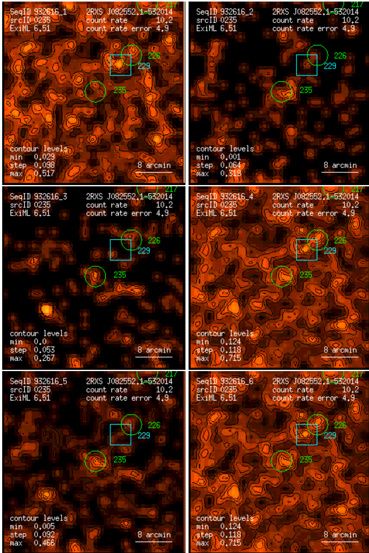
Figure 235: RASS 932616: detection 0235: band rate images, Gaussian filter: (1) PSPC channels 11 – 41, (2) 52 – 90, (3) 91 – 201, (4) 11 – 235, (5) 52 – 201, (6) 11 – 201. Broad band rates in counts/ks. Band rate contour levels in counts/ks/arcmin 2 .
