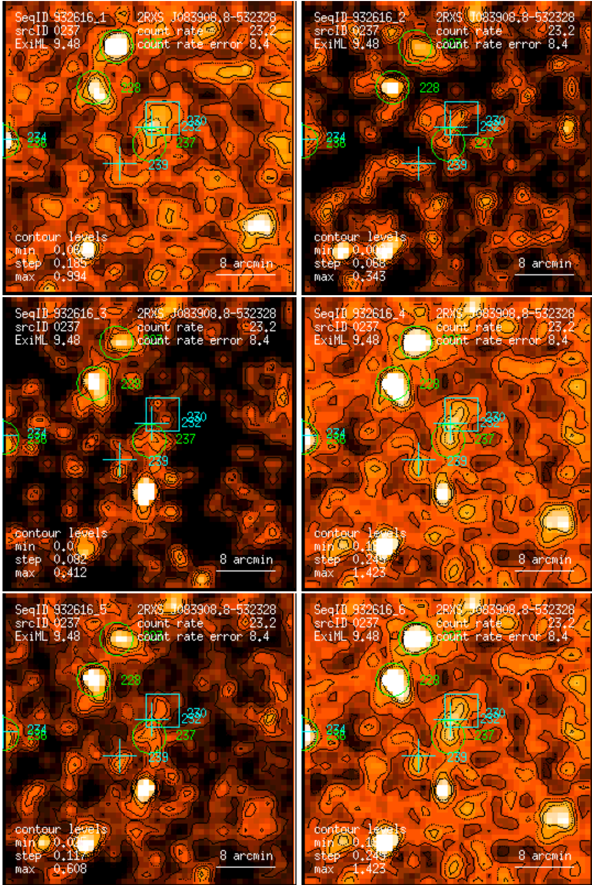
Figure 237: RASS 932616: detection 0237: band rate images, Gaussian filter: (1) PSPC channels 11 – 41, (2) 52 – 90, (3) 91 – 201, (4) 11 – 235, (5) 52 – 201, (6) 11 – 201. Broad band rates in counts/ks. Band rate contour levels in counts/ks/arcmin 2 .
