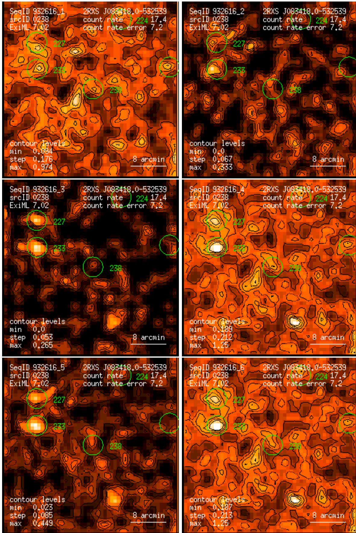
Figure 238: RASS 932616: detection 0238: band rate images, Gaussian filter: (1) PSPC channels 11 – 41, (2) 52 – 90, (3) 91 – 201, (4) 11 – 235, (5) 52 – 201, (6) 11 – 201. Broad band rates in counts/ks. Band rate contour levels in counts/ks/arcmin 2 .
