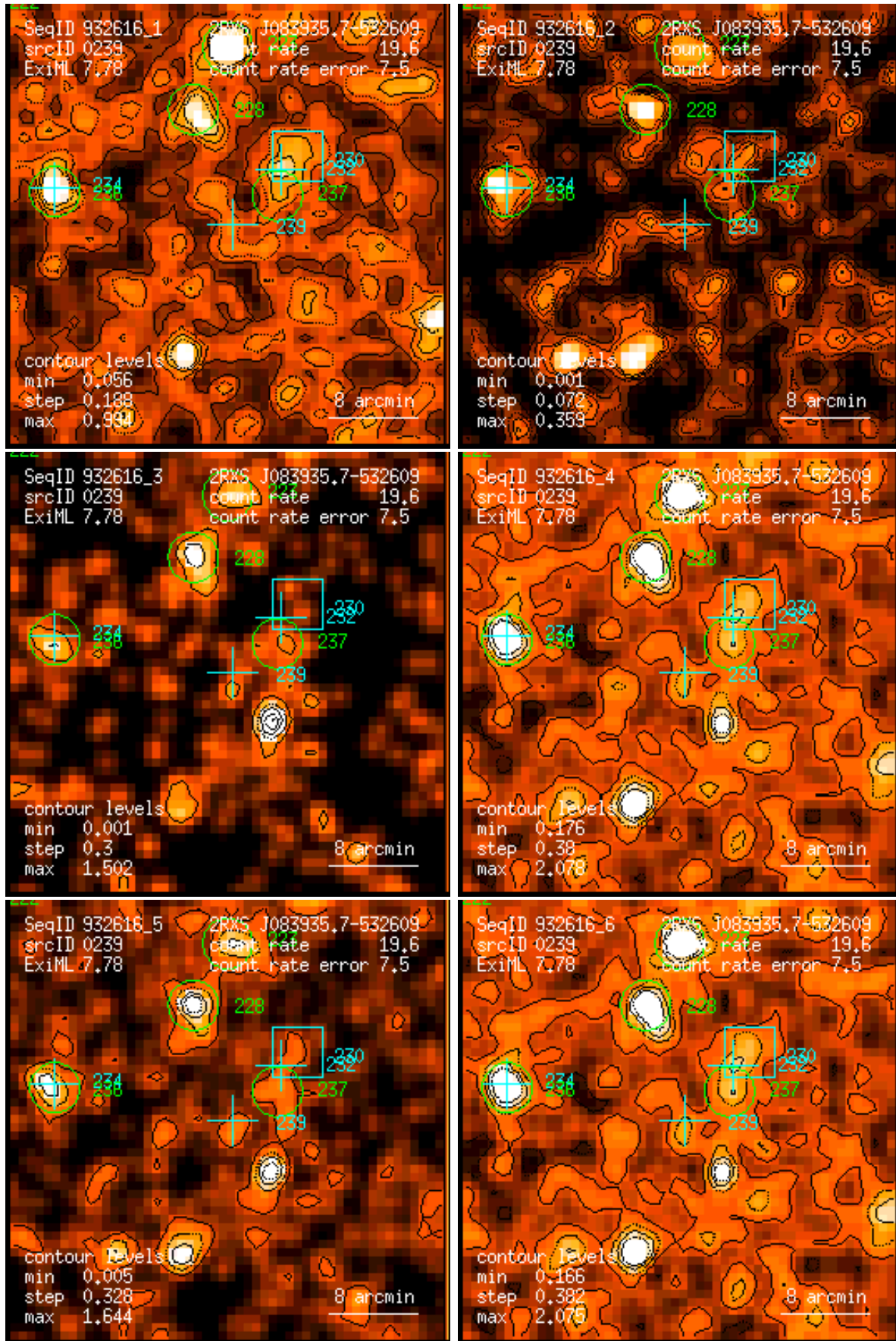
Figure 239: RASS 932616: detection 0239: band rate images, Gaussian filter: (1) PSPC channels 11 – 41, (2) 52 – 90, (3) 91 – 201, (4) 11 – 235, (5) 52 – 201, (6) 11 – 201. Broad band rates in counts/ks. Band rate contour levels in counts/ks/arcmin 2 .
