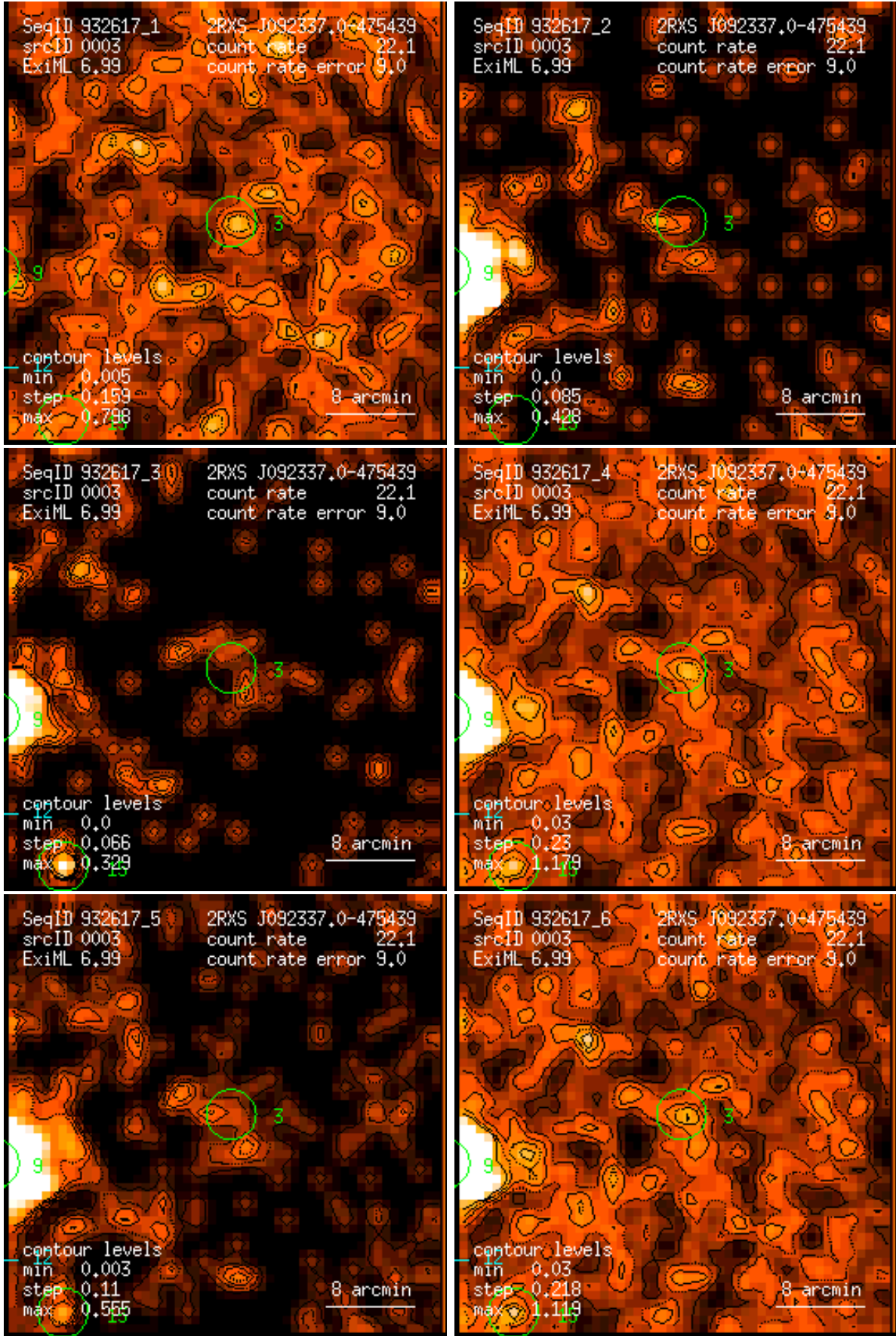
Figure 3: RASS 932617: detection 0003: band rate images, Gaussian filter: (1) PSPC channels 11 – 41, (2) 52 – 90, (3) 91 – 201, (4) 11 – 235, (5) 52 – 201, (6) 11 – 201. Broad band rates in counts/ks. Band rate contour levels in counts/ks/arcmin 2 .
