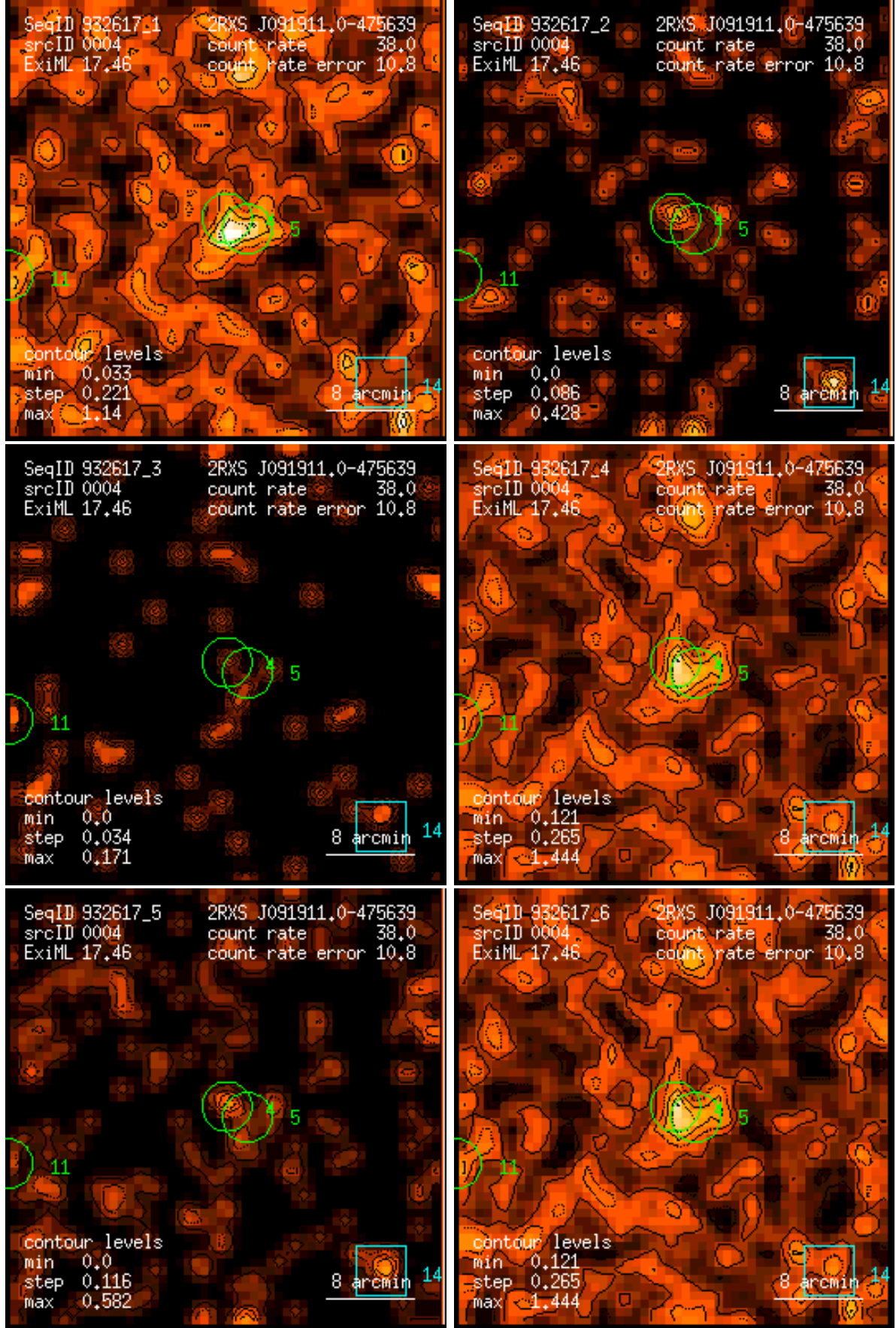
Figure 4: RASS 932617: detection 0004: band rate images, Gaussian filter: (1) PSPC channels 11 – 41, (2) 52 – 90, (3) 91 – 201, (4) 11 – 235, (5) 52 – 201, (6) 11 – 201. Broad band rates in counts/ks. Band rate contour levels in counts/ks/arcmin 2 .
