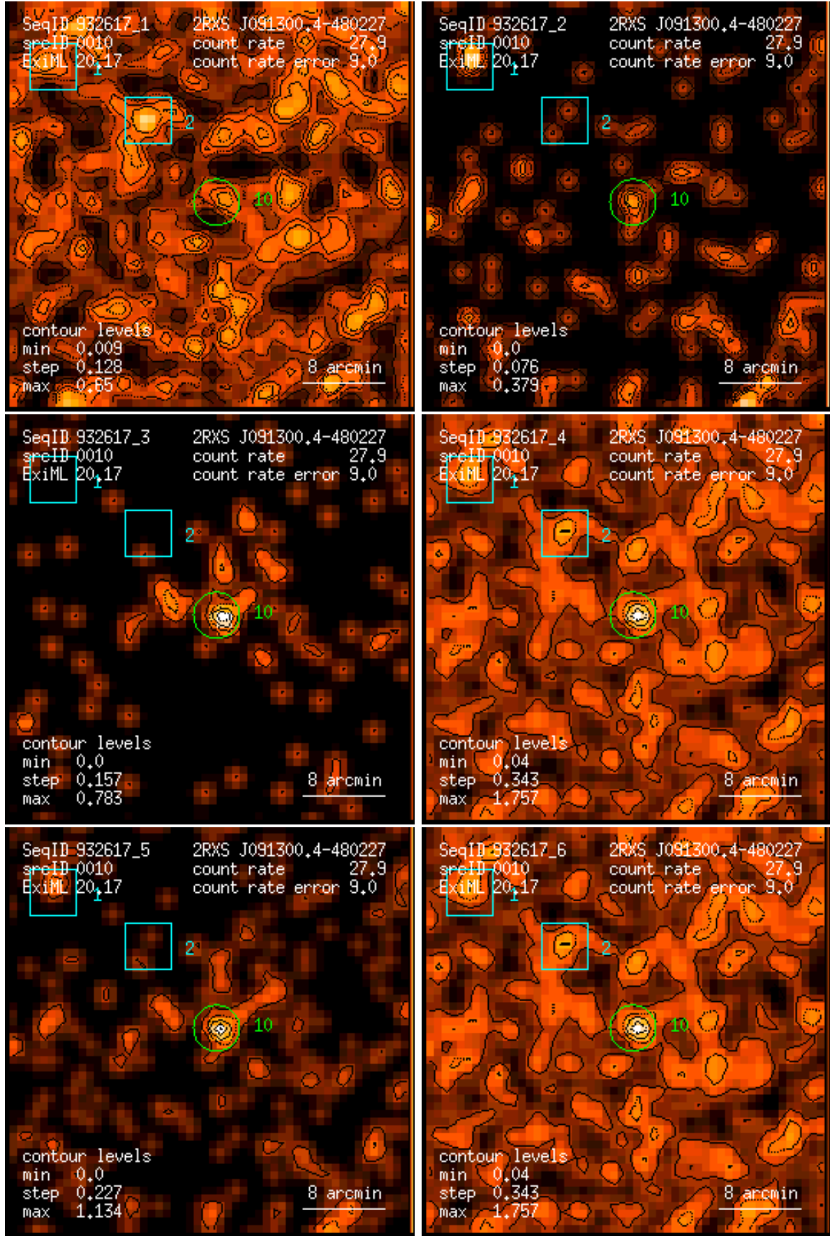
Figure 10: RASS 932617: detection 0010: band rate images, Gaussian filter: (1) PSPC channels 11 – 41, (2) 52 – 90, (3) 91 – 201, (4) 11 – 235, (5) 52 – 201, (6) 11 – 201. Broad band rates in counts/ks. Band rate contour levels in counts/ks/arcmin 2 .
