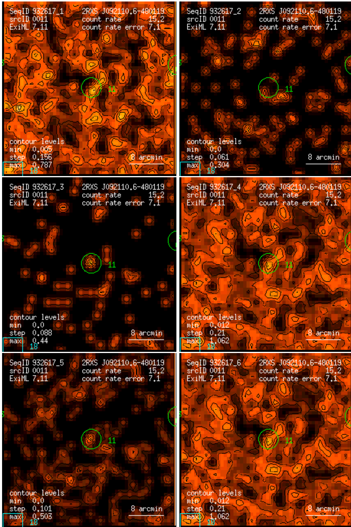
Figure 11: RASS 932617: detection 0011: band rate images, Gaussian filter: (1) PSPC channels 11 – 41, (2) 52 – 90, (3) 91 – 201, (4) 11 – 235, (5) 52 – 201, (6) 11 – 201. Broad band rates in counts/ks. Band rate contour levels in counts/ks/arcmin 2 .
