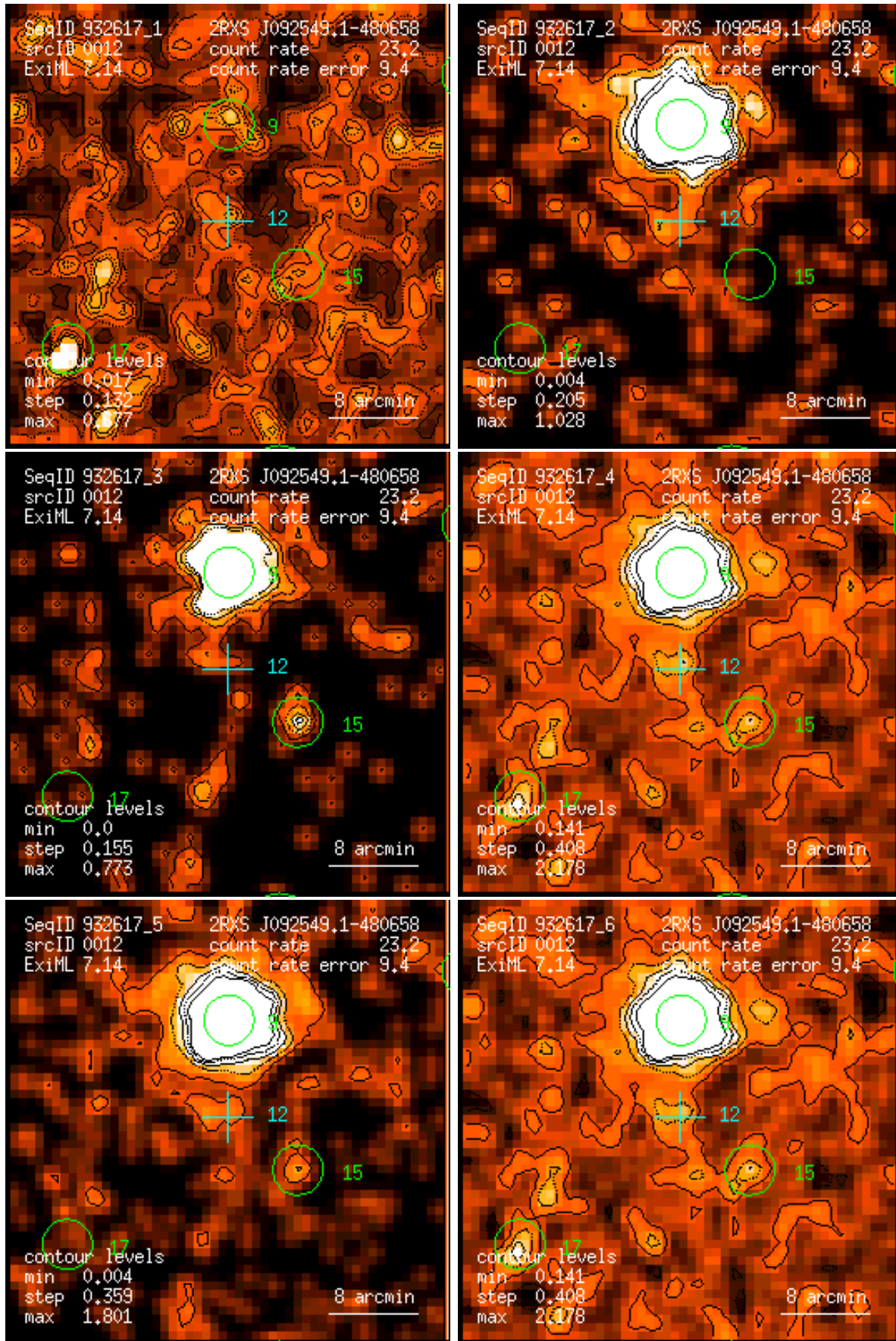
Figure 12: RASS 932617: detection 0012: band rate images, Gaussian filter: (1) PSPC channels 11 – 41, (2) 52 – 90, (3) 91 – 201, (4) 11 – 235, (5) 52 – 201, (6) 11 – 201. Broad band rates in counts/ks. Band rate contour levels in counts/ks/arcmin 2 .
