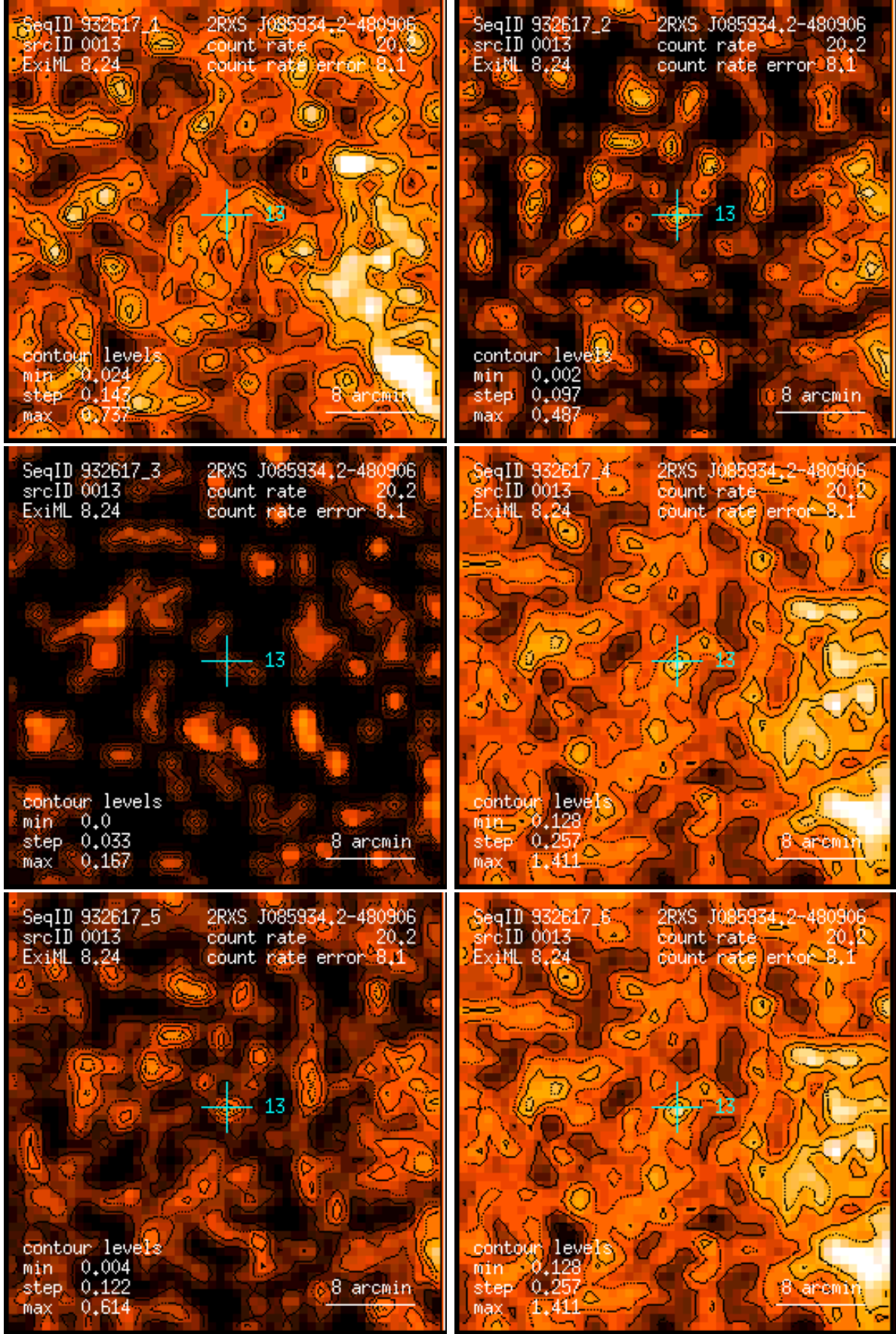
Figure 13: RASS 932617: detection 0013: band rate images, Gaussian filter: (1) PSPC channels 11 – 41, (2) 52 – 90, (3) 91 – 201, (4) 11 – 235, (5) 52 – 201, (6) 11 – 201. Broad band rates in counts/ks. Band rate contour levels in counts/ks/arcmin 2 .
