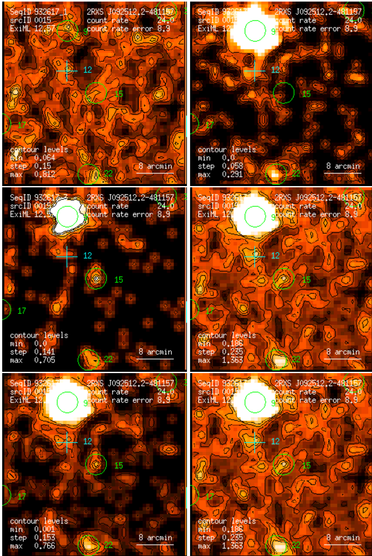
Figure 15: RASS 932617: detection 0015: band rate images, Gaussian filter: (1) PSPC channels 11 – 41, (2) 52 – 90, (3) 91 – 201, (4) 11 – 235, (5) 52 – 201, (6) 11 – 201. Broad band rates in counts/ks. Band rate contour levels in counts/ks/arcmin 2 .
