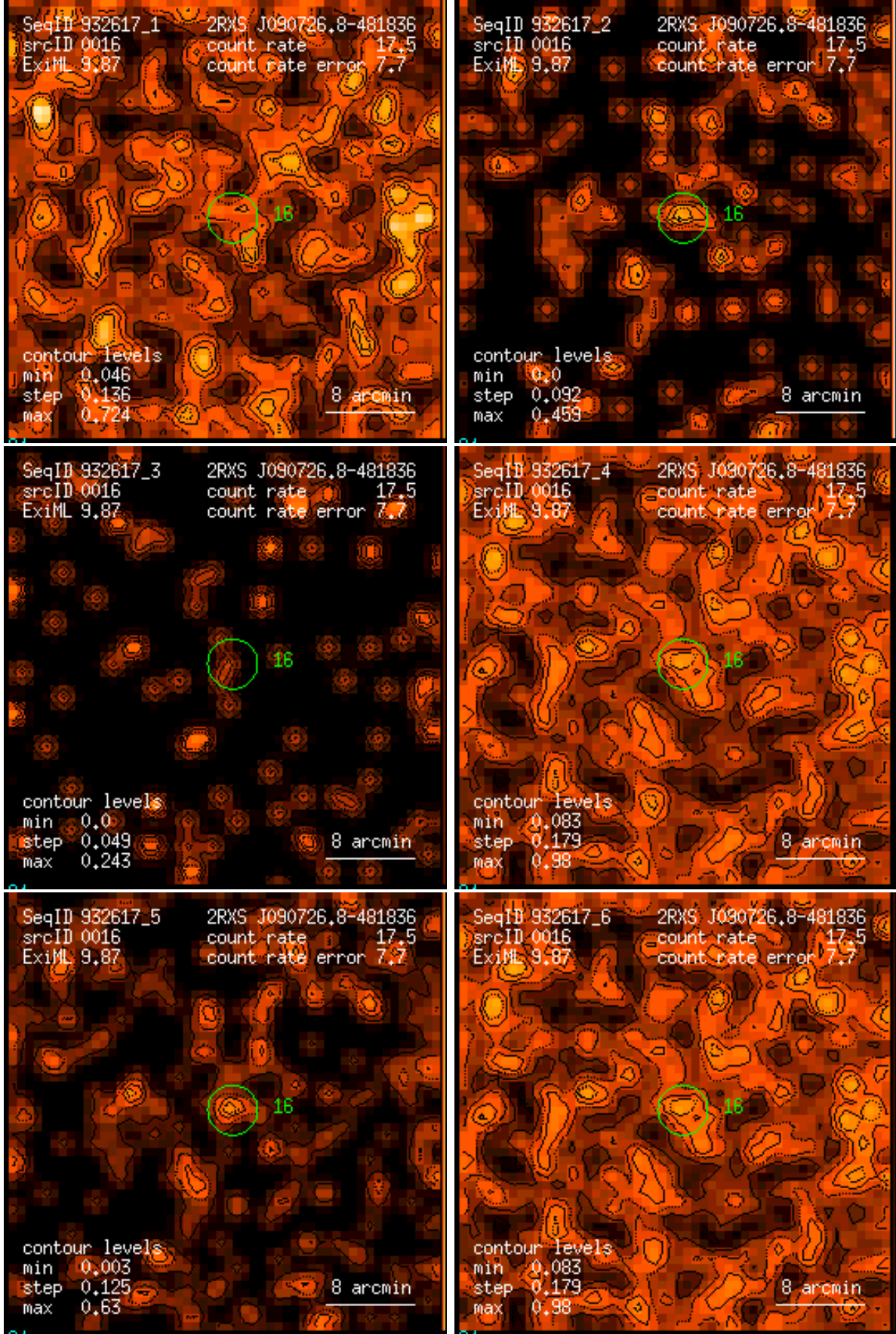
Figure 16: RASS 932617: detection 0016: band rate images, Gaussian filter: (1) PSPC channels 11 – 41, (2) 52 – 90, (3) 91 – 201, (4) 11 – 235, (5) 52 – 201, (6) 11 – 201. Broad band rates in counts/ks. Band rate contour levels in counts/ks/arcmin 2 .
