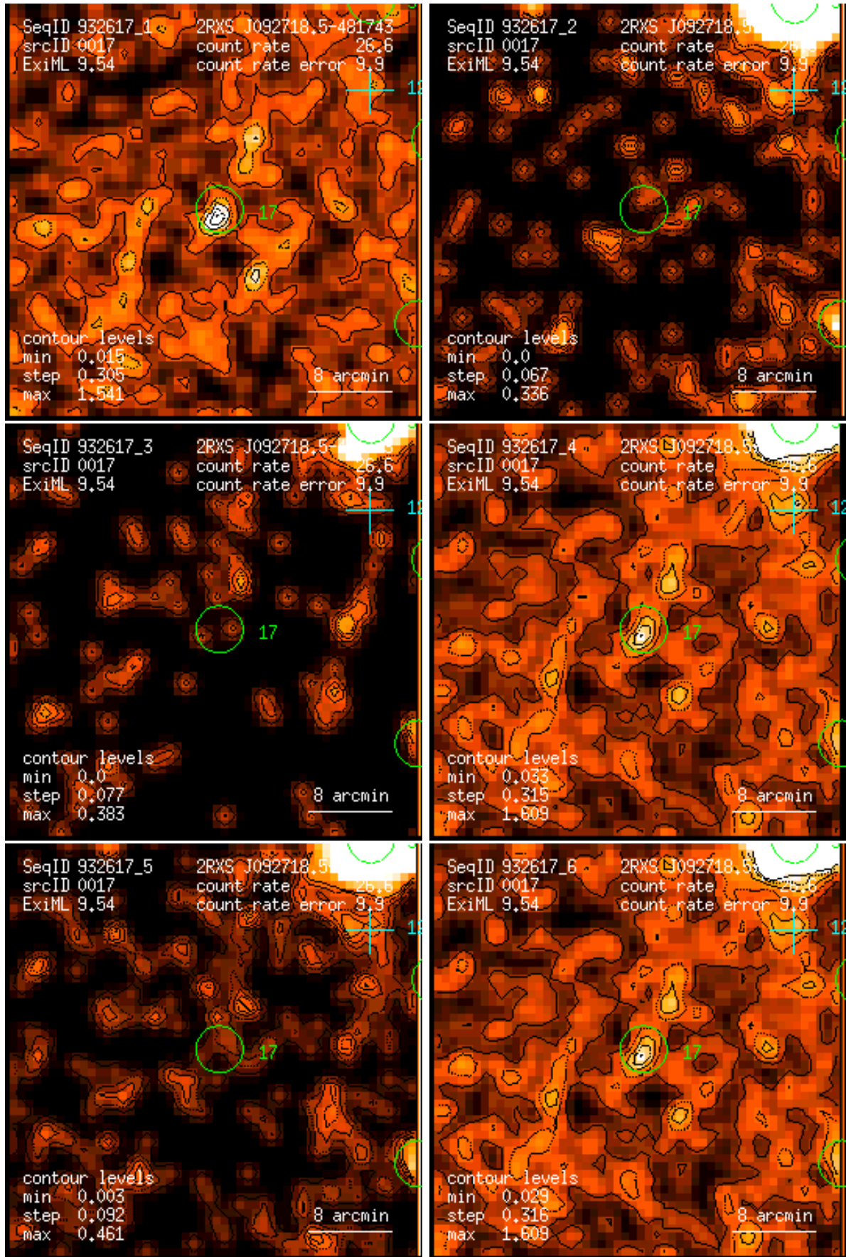
Figure 17: RASS 932617: detection 0017: band rate images, Gaussian filter: (1) PSPC channels 11 – 41, (2) 52 – 90, (3) 91 – 201, (4) 11 – 235, (5) 52 – 201, (6) 11 – 201. Broad band rates in counts/ks. Band rate contour levels in counts/ks/arcmin 2 .
