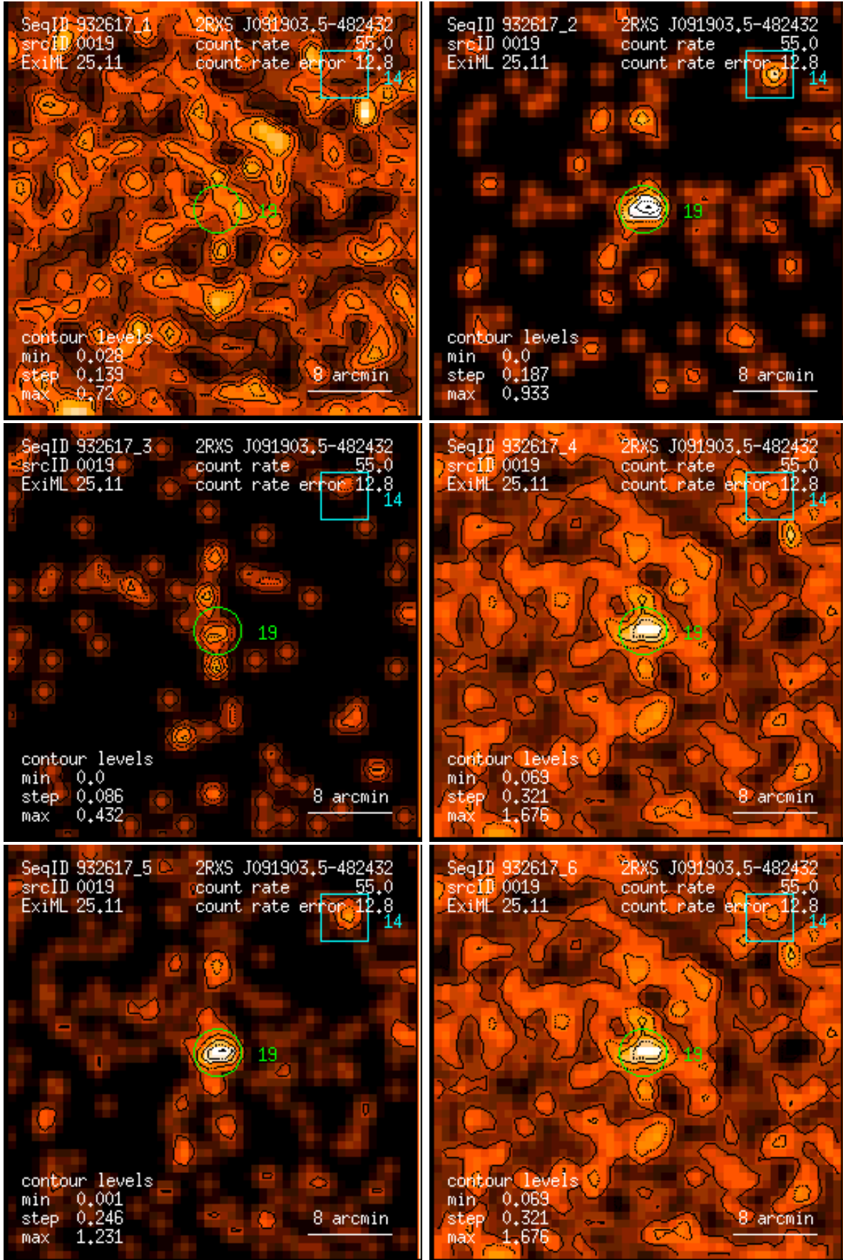
Figure 19: RASS 932617: detection 0019: band rate images, Gaussian filter: (1) PSPC channels 11 – 41, (2) 52 – 90, (3) 91 – 201, (4) 11 – 235, (5) 52 – 201, (6) 11 – 201. Broad band rates in counts/ks. Band rate contour levels in counts/ks/arcmin 2 .
