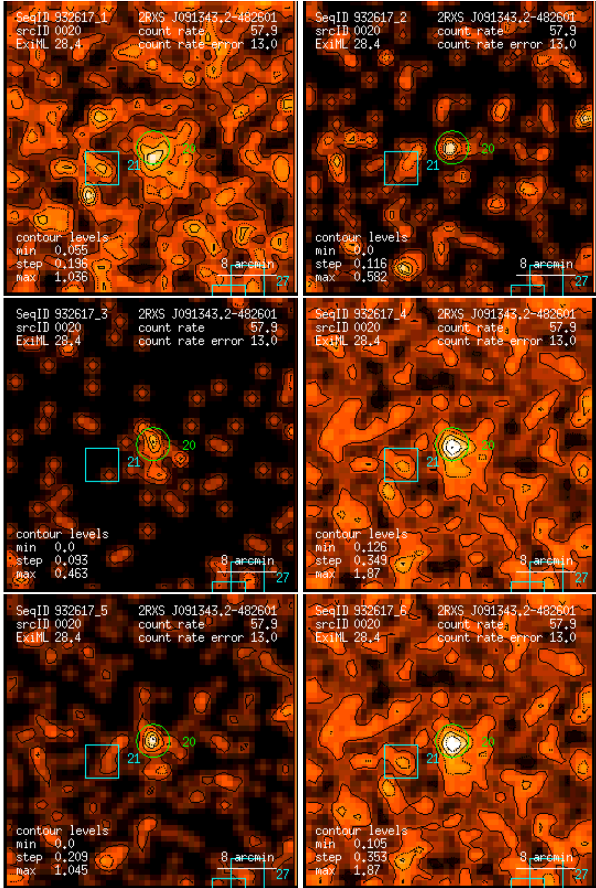
Figure 20: RASS 932617: detection 0020: band rate images, Gaussian filter: (1) PSPC channels 11 – 41, (2) 52 – 90, (3) 91 – 201, (4) 11 – 235, (5) 52 – 201, (6) 11 – 201. Broad band rates in counts/ks. Band rate contour levels in counts/ks/arcmin 2 .
