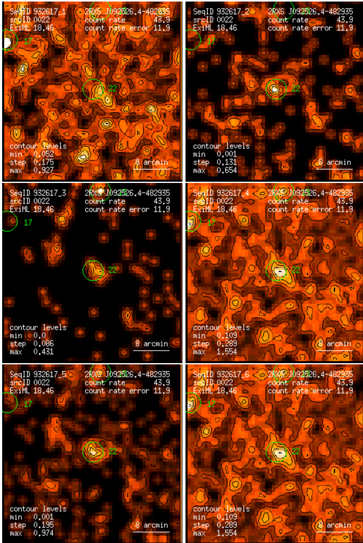
Figure 22: RASS 932617: detection 0022: band rate images, Gaussian filter: (1) PSPC channels 11 – 41, (2) 52 – 90, (3) 91 – 201, (4) 11 – 235, (5) 52 – 201, (6) 11 – 201. Broad band rates in counts/ks. Band rate contour levels in counts/ks/arcmin 2 .
