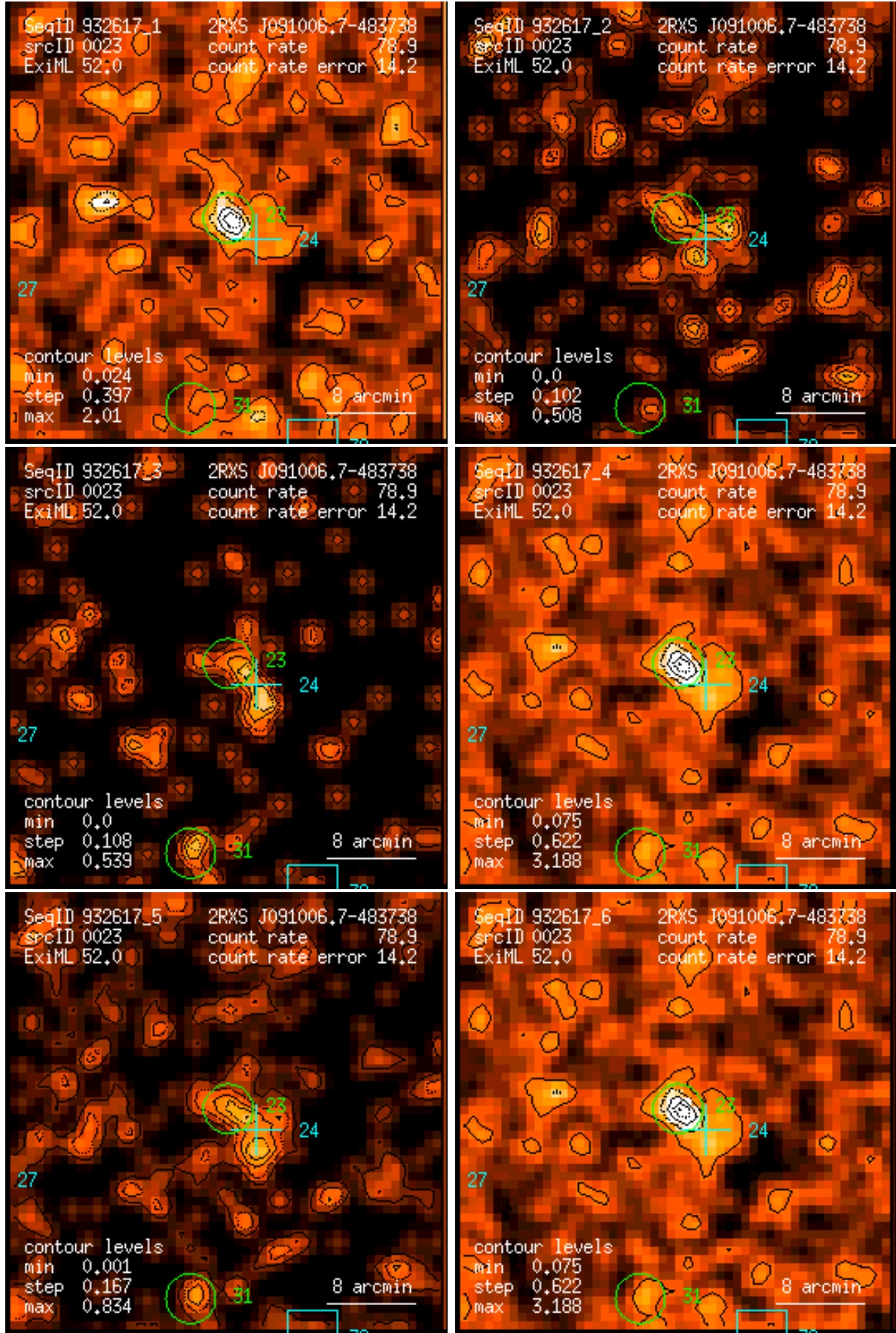
Figure 23: RASS 932617: detection 0023: band rate images, Gaussian filter: (1) PSPC channels 11 – 41, (2) 52 – 90, (3) 91 – 201, (4) 11 – 235, (5) 52 – 201, (6) 11 – 201. Broad band rates in counts/ks. Band rate contour levels in counts/ks/arcmin 2 .
