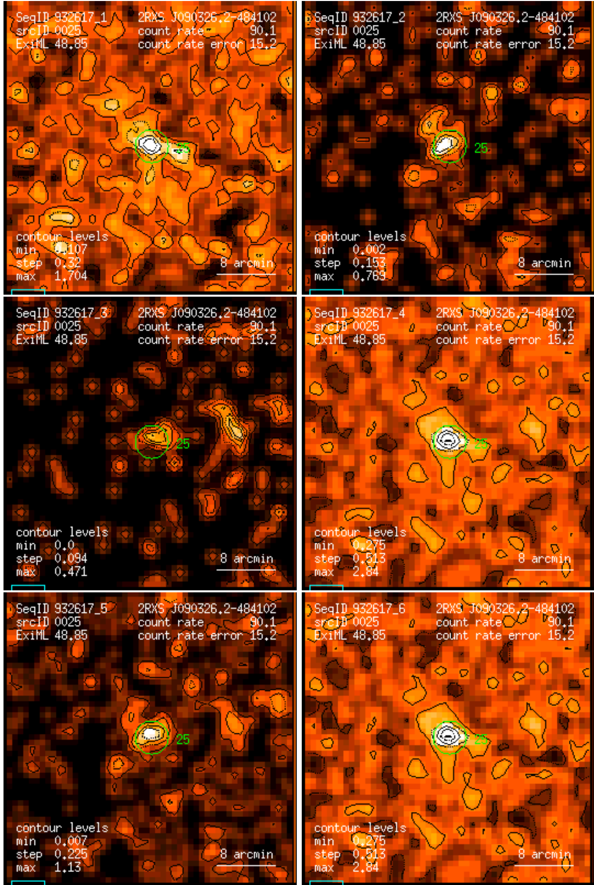
Figure 25: RASS 932617: detection 0025: band rate images, Gaussian filter: (1) PSPC channels 11 – 41, (2) 52 – 90, (3) 91 – 201, (4) 11 – 235, (5) 52 – 201, (6) 11 – 201. Broad band rates in counts/ks. Band rate contour levels in counts/ks/arcmin 2 .
