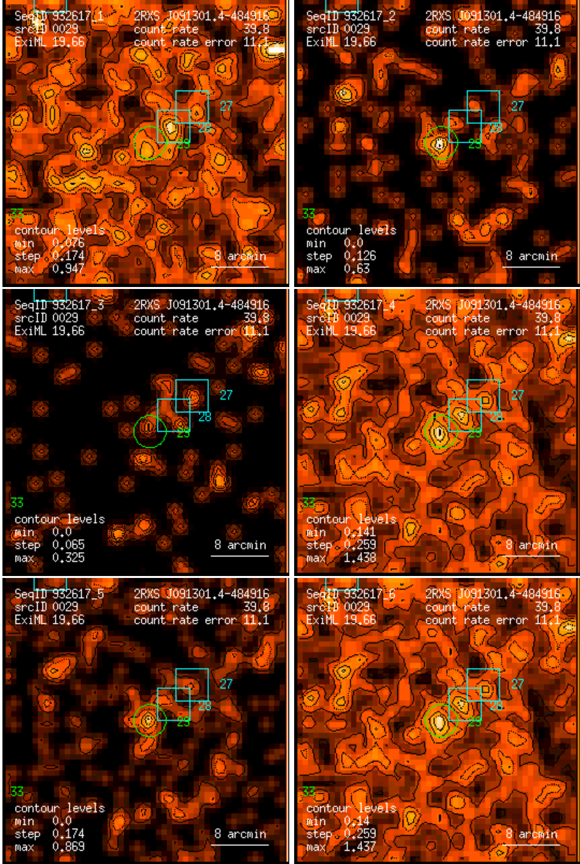
Figure 29: RASS 932617: detection 0029: band rate images, Gaussian filter: (1) PSPC channels 11 – 41, (2) 52 – 90, (3) 91 – 201, (4) 11 – 235, (5) 52 – 201, (6) 11 – 201. Broad band rates in counts/ks. Band rate contour levels in counts/ks/arcmin 2 .
