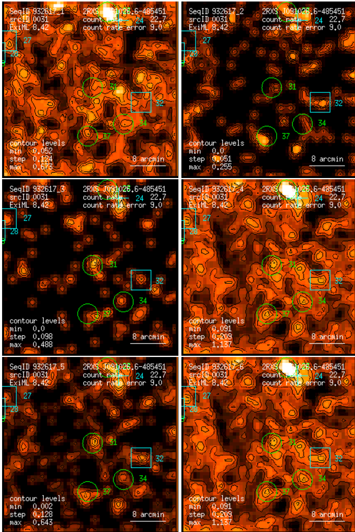
Figure 31: RASS 932617: detection 0031: band rate images, Gaussian filter: (1) PSPC channels 11 – 41, (2) 52 – 90, (3) 91 – 201, (4) 11 – 235, (5) 52 – 201, (6) 11 – 201. Broad band rates in counts/ks. Band rate contour levels in counts/ks/arcmin 2 .
