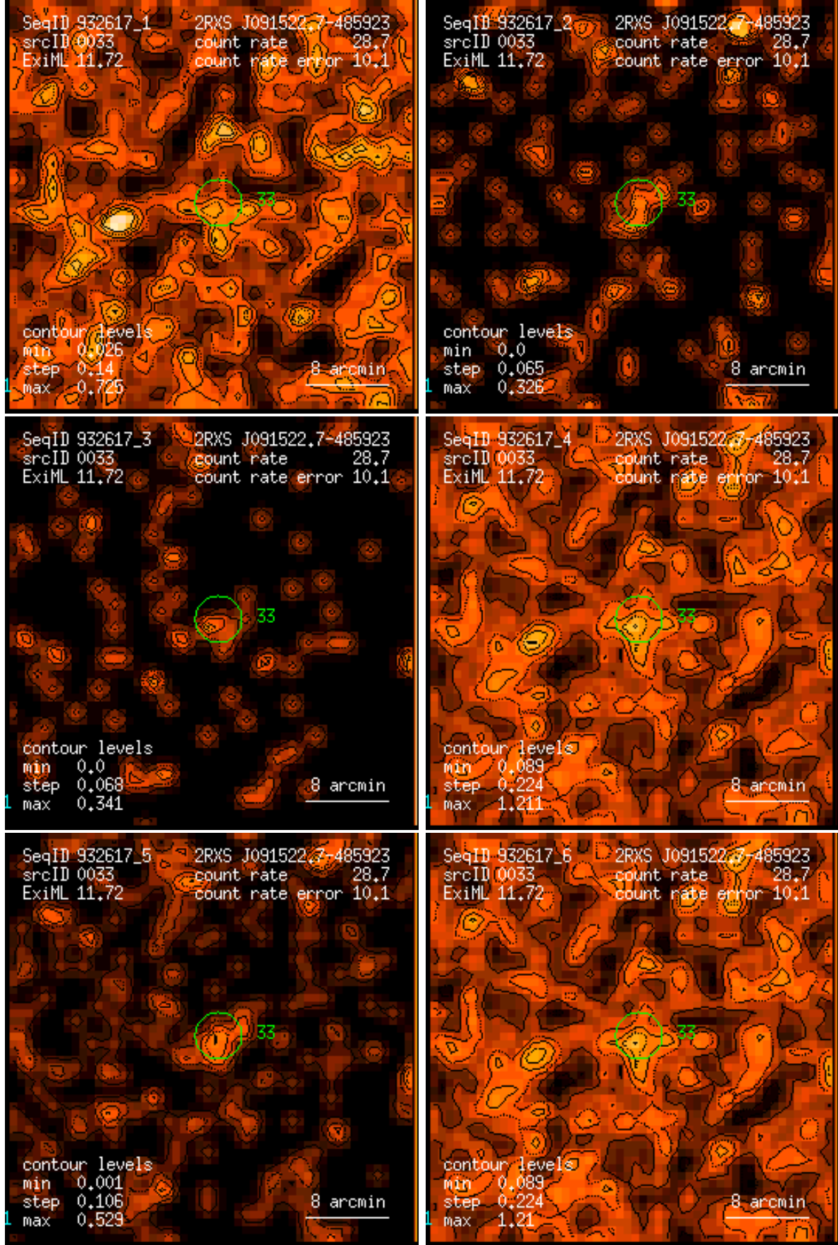
Figure 33: RASS 932617: detection 0033: band rate images, Gaussian filter: (1) PSPC channels 11 – 41, (2) 52 – 90, (3) 91 – 201, (4) 11 – 235, (5) 52 – 201, (6) 11 – 201. Broad band rates in counts/ks. Band rate contour levels in counts/ks/arcmin 2 .
