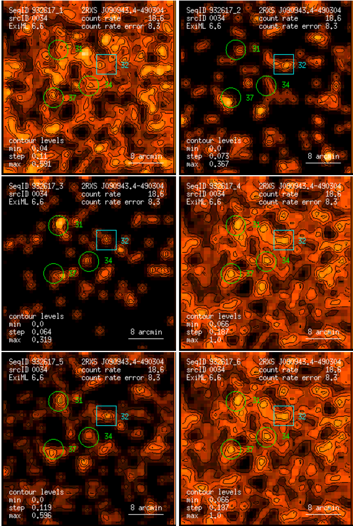
Figure 34: RASS 932617: detection 0034: band rate images, Gaussian filter: (1) PSPC channels 11 – 41, (2) 52 – 90, (3) 91 – 201, (4) 11 – 235, (5) 52 – 201, (6) 11 – 201. Broad band rates in counts/ks. Band rate contour levels in counts/ks/arcmin 2 .
