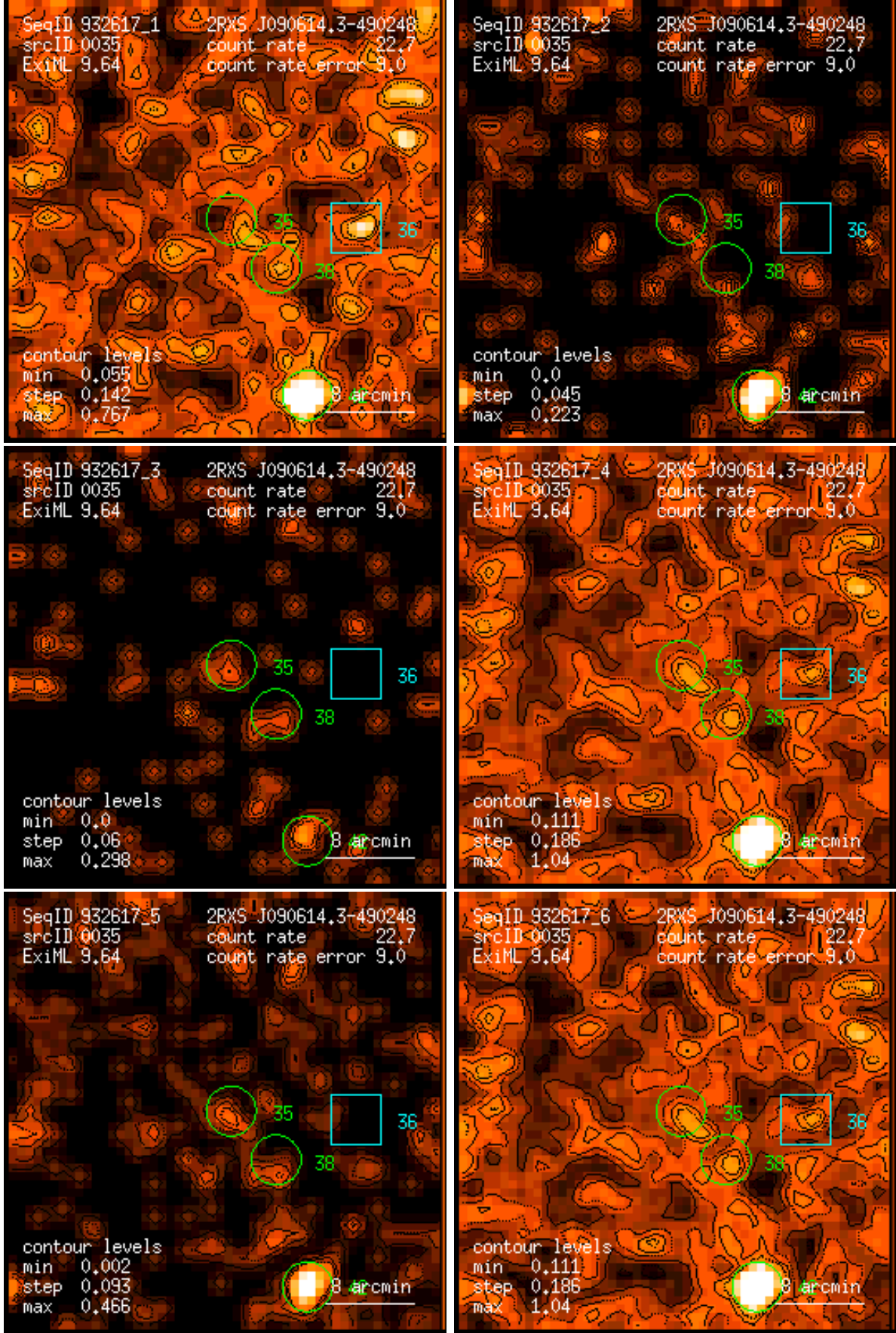
Figure 35: RASS 932617: detection 0035: band rate images, Gaussian filter: (1) PSPC channels 11 – 41, (2) 52 – 90, (3) 91 – 201, (4) 11 – 235, (5) 52 – 201, (6) 11 – 201. Broad band rates in counts/ks. Band rate contour levels in counts/ks/arcmin 2 .
