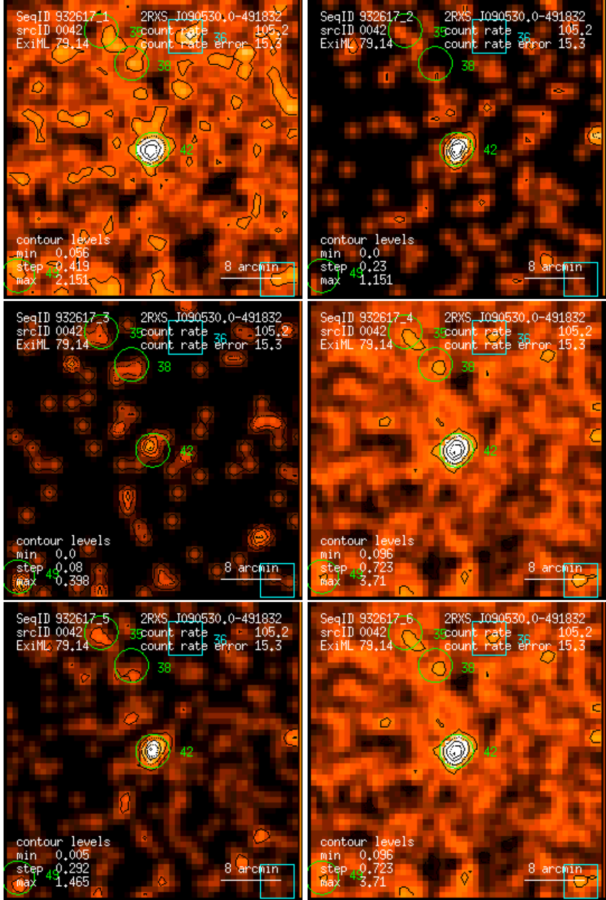
Figure 42: RASS 932617: detection 0042: band rate images, Gaussian filter: (1) PSPC channels 11 – 41, (2) 52 – 90, (3) 91 – 201, (4) 11 – 235, (5) 52 – 201, (6) 11 – 201. Broad band rates in counts/ks. Band rate contour levels in counts/ks/arcmin 2 .
